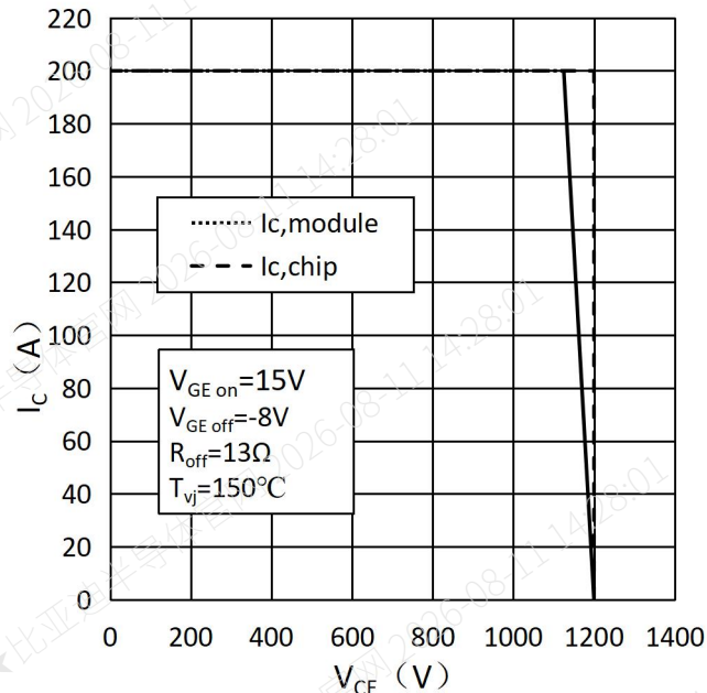
图 8 反偏安全工作区 Fig.8 Reverse Bias Safe Operating Area (RBSOA)
