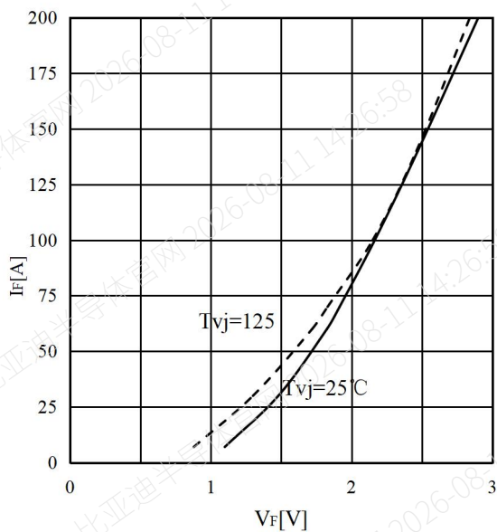
Fig.9 FWD Forward Characteristics
