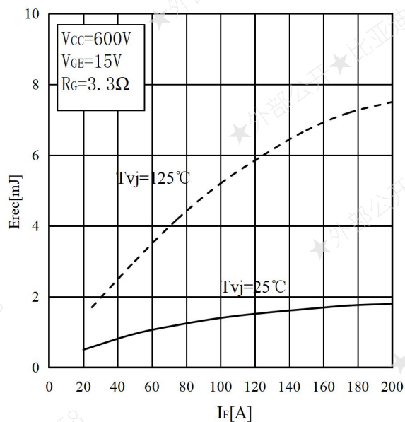
Fig.10 Typ. Switching Losses Diode-Inverter
