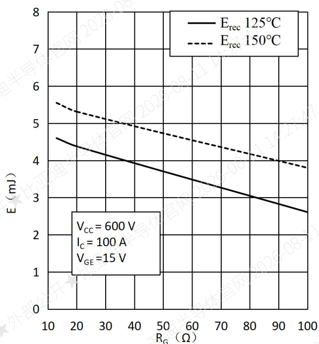
Fig.9 Switching Loss of Diode vs. Gate Resistor-Inverter
