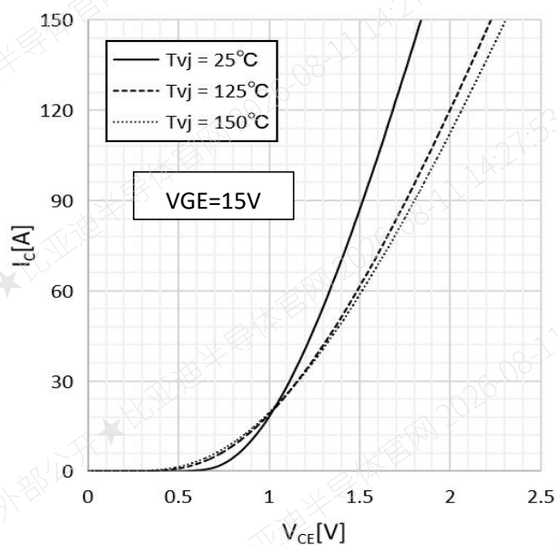
Fig.1 Typ. On-state Characteristics
