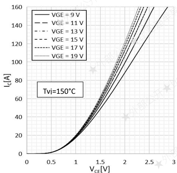
Fig.3 Typ. Output Characteristics
