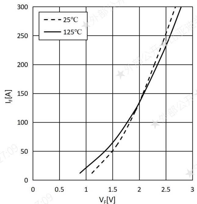
Fig.6 FWD Forward Characteristics
