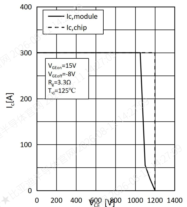
Fig.8 Reverse Bias Safe Operating Area (RBSOA)
