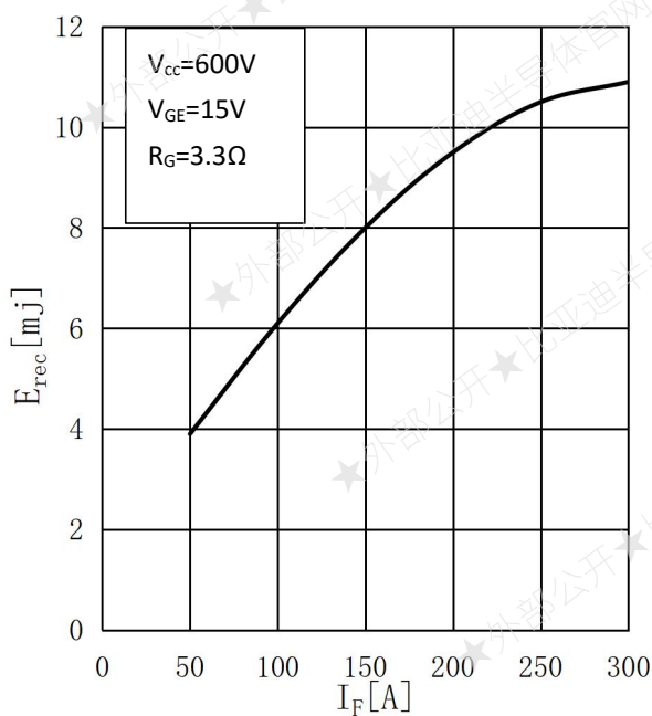
Fig.7 Typ. Switching Losses Diode-Inverter
