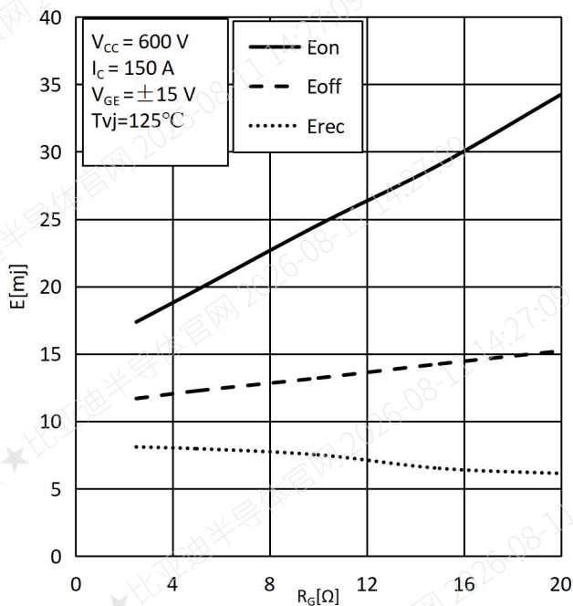
Fig.5 Switching Loss vs. Gate Resistor
