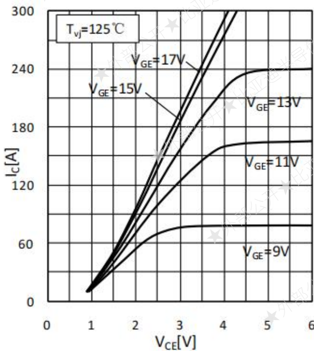
Fig.3 Typ. Output Characteristics
