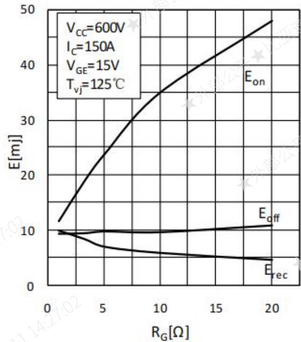
Fig.6 Switching Loss vs. Gate Resistor 图 6 开关损耗和门极电阻
