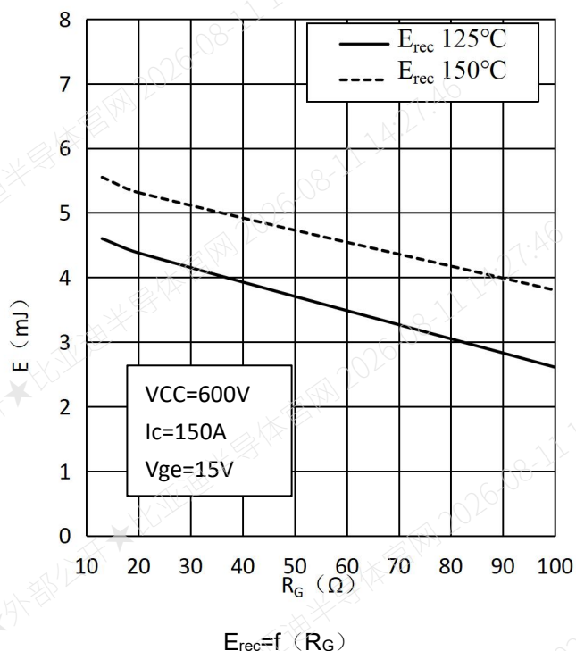
Fig.9 Switching Loss of Diode vs. Gate Resistor-Inverter
