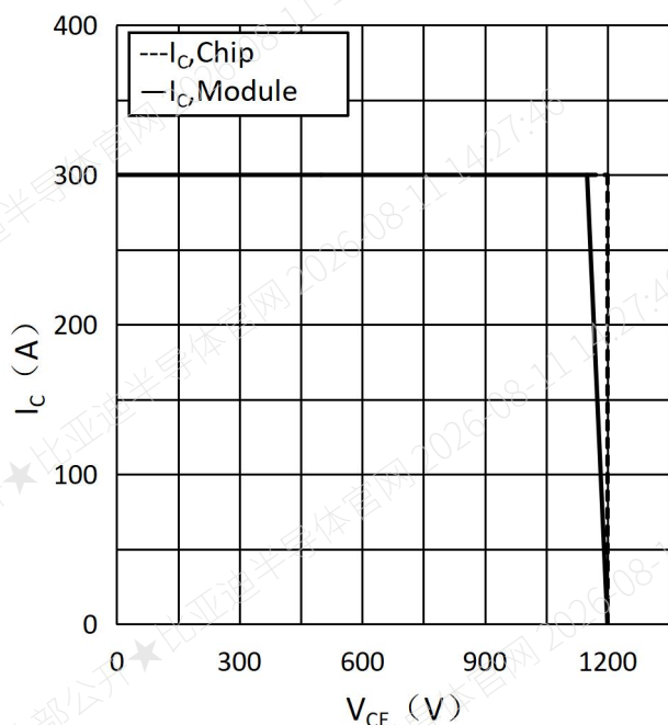
Fig.5 Reverse Bias Safe Operating Area (RBSOA)
