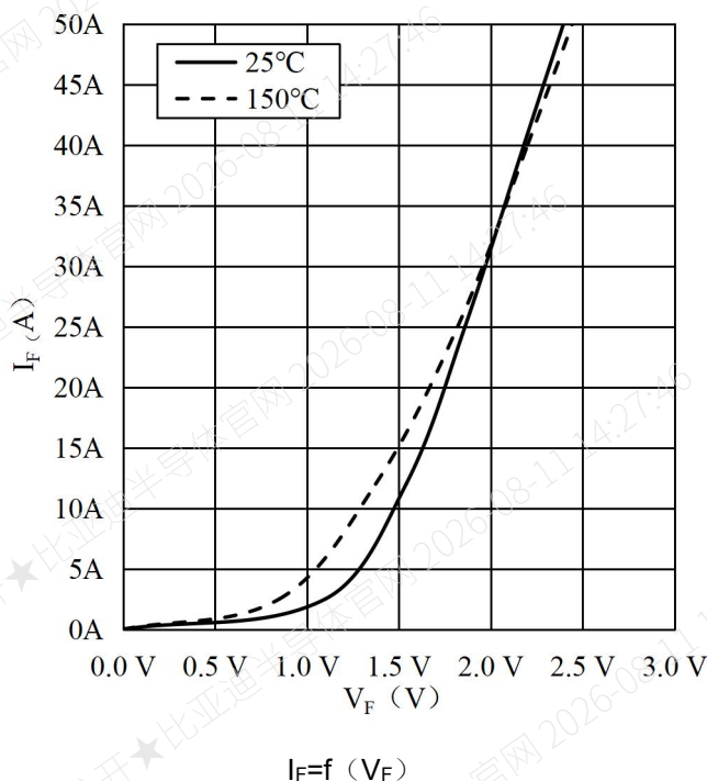
Fig. 12 Forward Characteristics of Diode-Brake-Chopper
