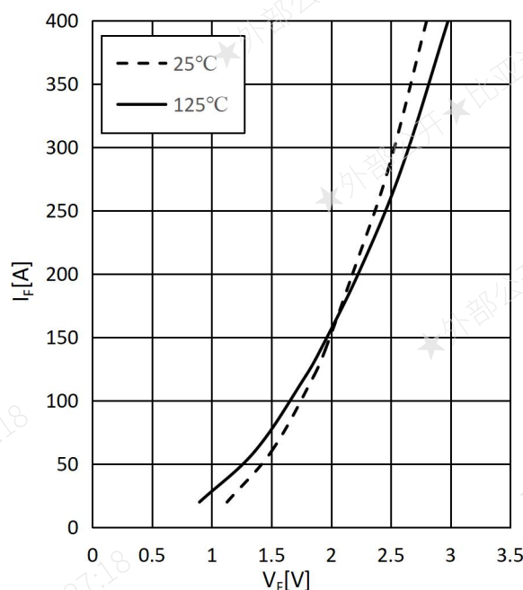
Fig.6 FWD Forward Characteristics
