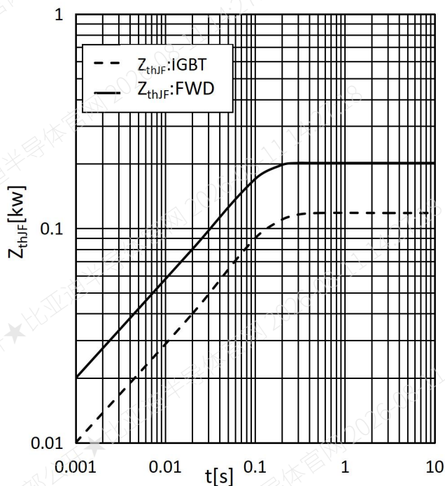
Fig.9 Typ. Transient Thermal Impedance
