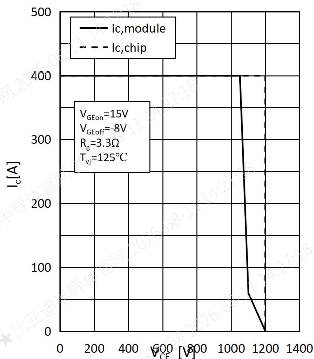
Fig.8 Reverse Bias Safe Operating Area (RBSOA)
