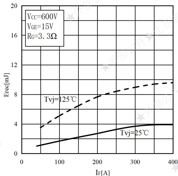
Fig.10 Typ. Switching Losses Diode-Inverter
