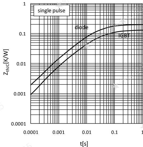
Fig.14 Typ. Transient Thermal Impedance
