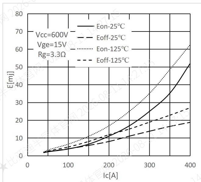
Fig.4 Switching Loss vs. Collector Current
