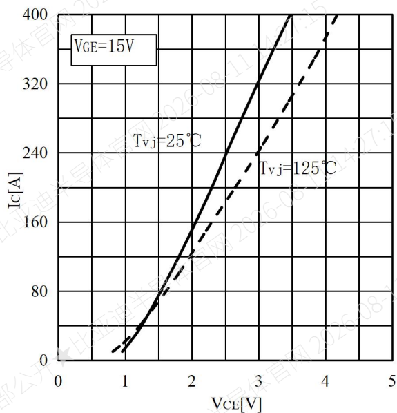
Fig.1 Typ. On-state Characteristics
