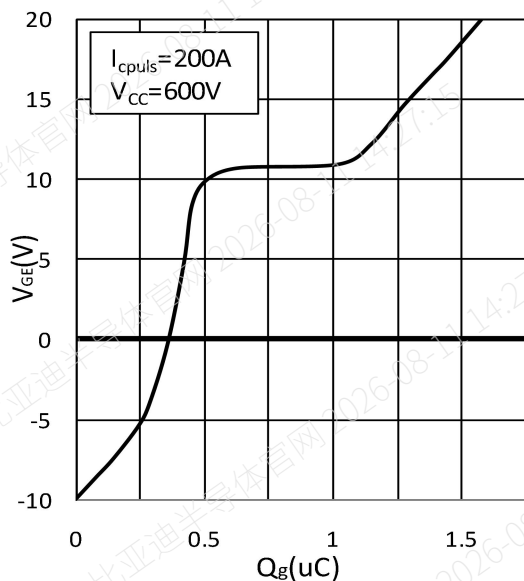
Fig.13 Typ. Gate Charge Characteristics
