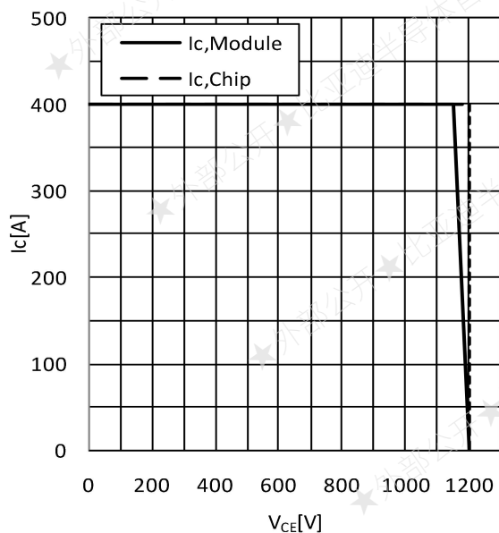
Fig.15 Reverse Bias Safe Operating Area (RBSOA)
