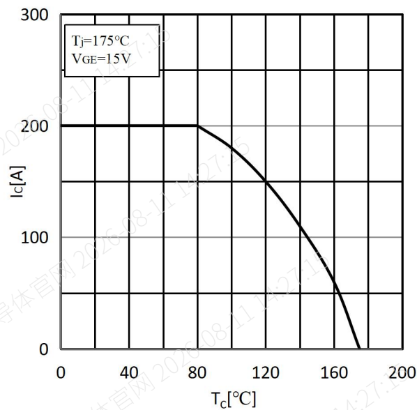
Fig.12 Rate Current vs. Temperature (Tc)
