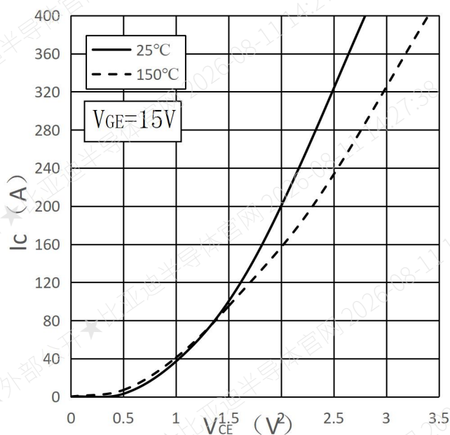
Fig.1 Typ. Output Characteristics-Inverter
