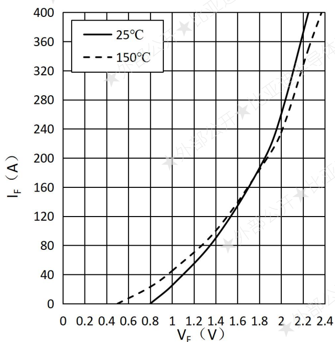
Fig.7 Typ. Forward Characteristics of Diode-Inverter
