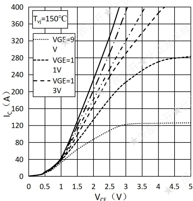
Fig.3 Typ. Output Characteristics-Inverter
