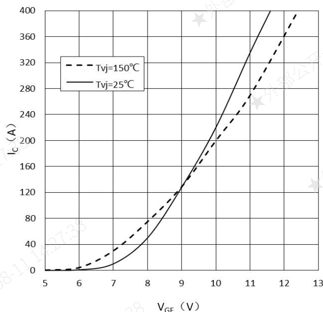
Fig.2 Typ. Transfer Characteristics-Inverter
