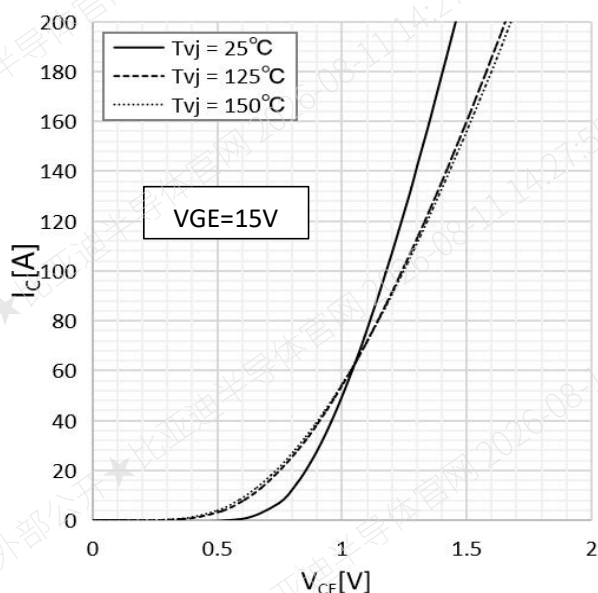
Fig.1 Typ. On-state Characteristics IGBT, T1 T4
