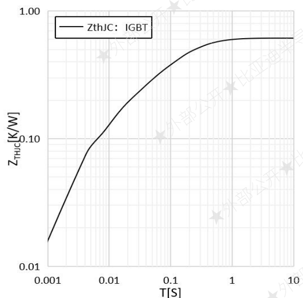
Fig.19 Typ. transient thermal impedance IGBT T2 T3
