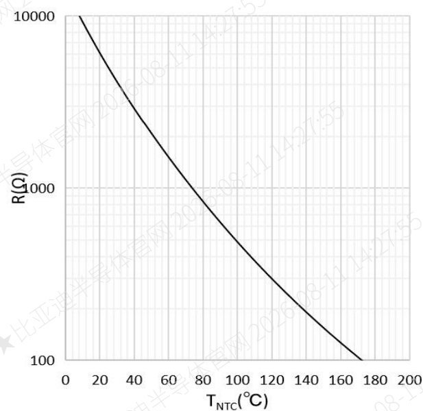
Fig.20 Typ. NTC-Temperature Characteristics
