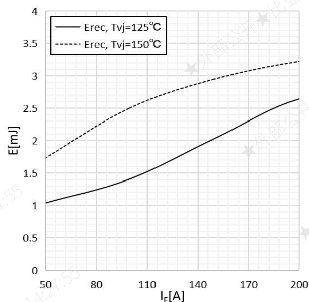
Fig.14 Reverse recovery Energy
