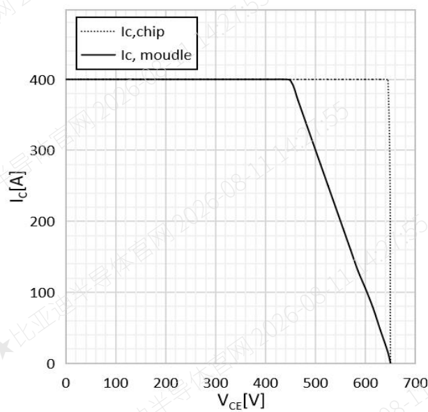
Fig.16 Reverse Bias Safe Operating Area IGBT, T2 T3
