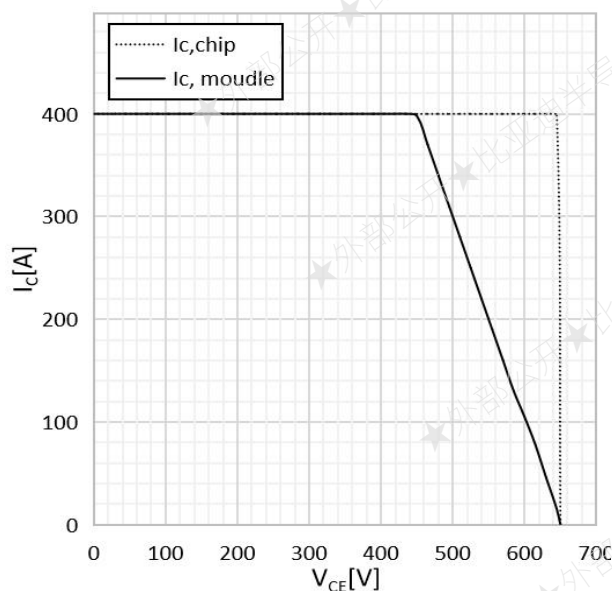
Fig.15 Reverse Bias Safe Operating Area IGBT, T1 T4
