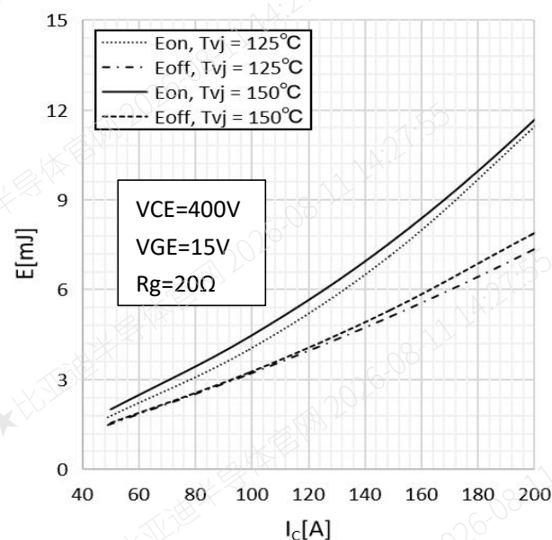
Fig.4 Switching Loss vs. Collector Current
