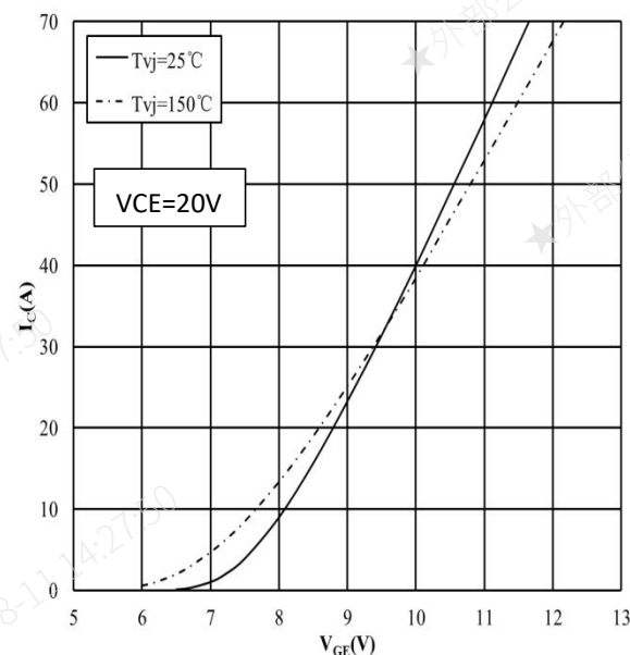
Fig.2 Typ. Transfer Characteristics
