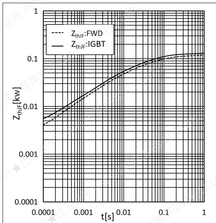
Fig.9 Typ. Transient Thermal Impedance
