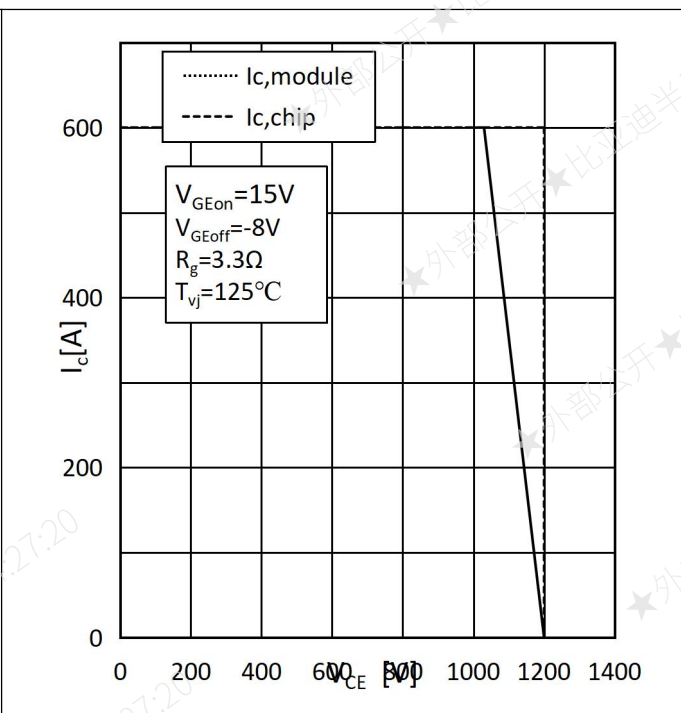
Fig.10 Reverse Bias Safe Operating Area (RBSOA)
