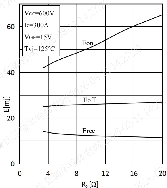
Fig.5 Switching Loss vs. Gate Resistor 图 5 开关损耗和门极电阻
