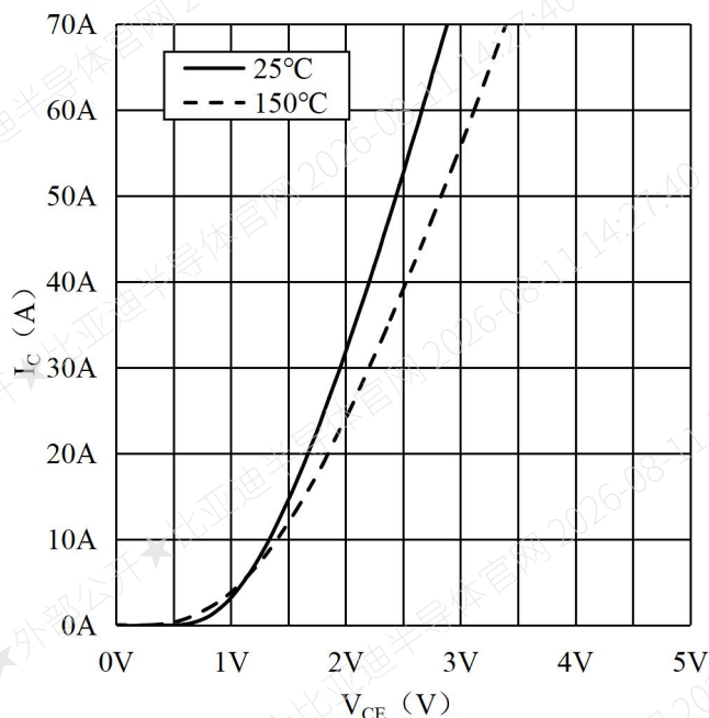
Fig.1 Typ. Output Characteristics-Inverter
