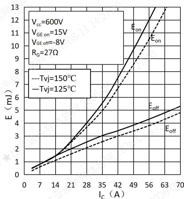
Fig.4 Switching Loss vs. Collector Current-Inverter
