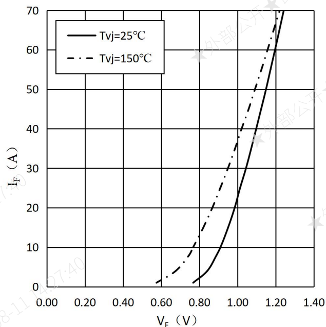
Fig.10 Forward Characteristics of Diode-Rectifier
