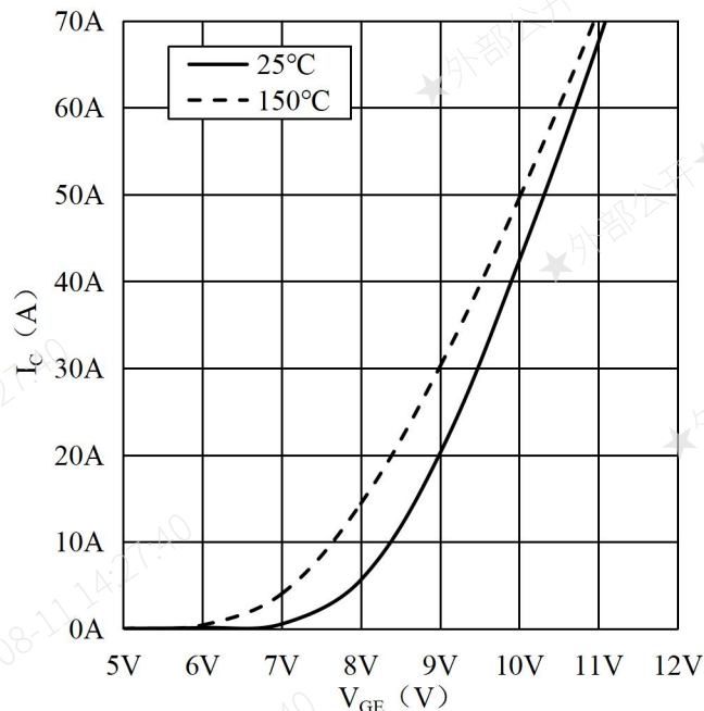
Fig.2 Typ. Transfer Characteristics-Inverter
