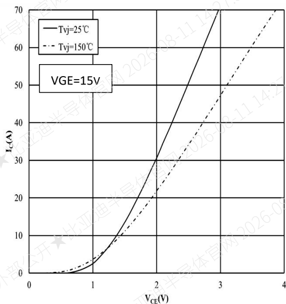
Fig.1 Typ. On-state Characteristics
