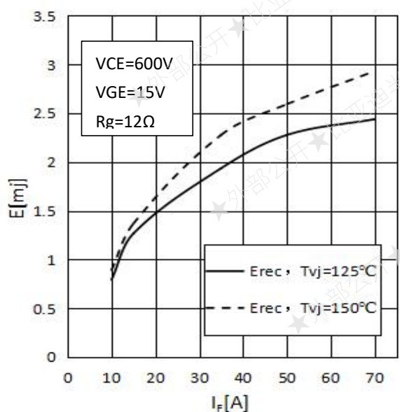
Fig.7 Reverse recovery Energy
