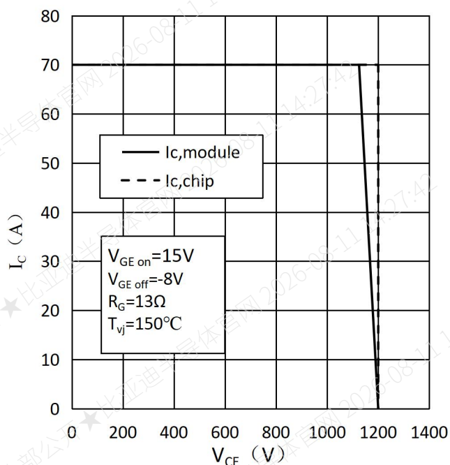
Fig.5 Reverse Bias Safe Operating Area (RBSOA) -Inverter
