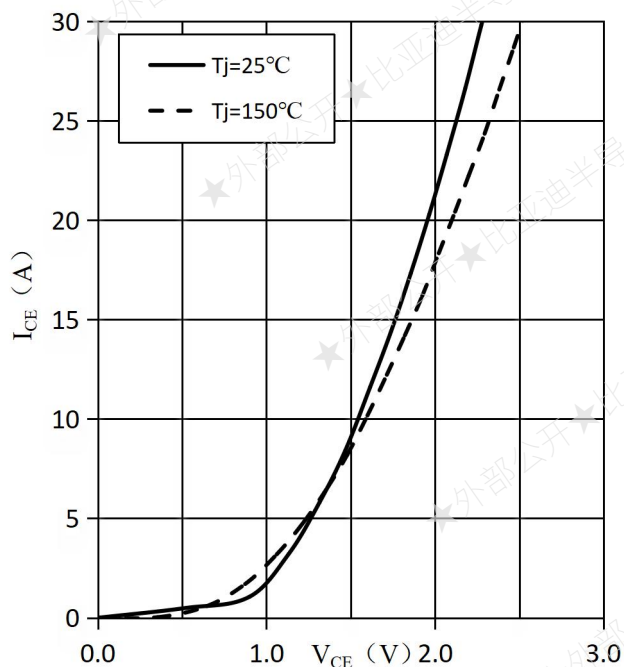
Fig.11 Typ. Output Characteristics, Brake-Chopper
