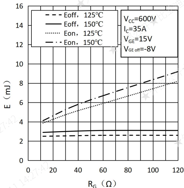
Fig.6 Switching Loss of IGBT vs. Gate Resistor - Inverter
