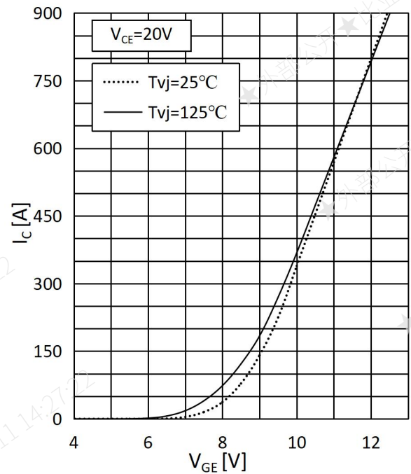
Fig.2 Transfer Characteristics
