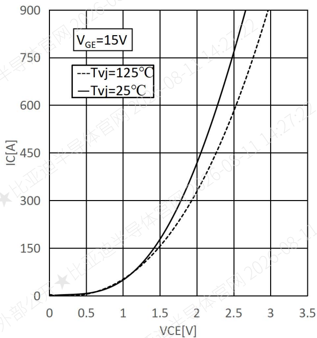
Fig.1 Output Characteristics
