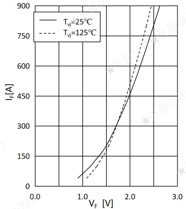
Fig.6 Forward Characteristics
