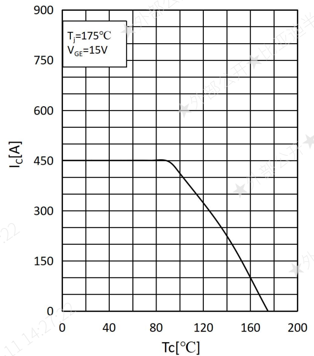
Fig. 10 Rate Current vs. Temperature ( T_c )
