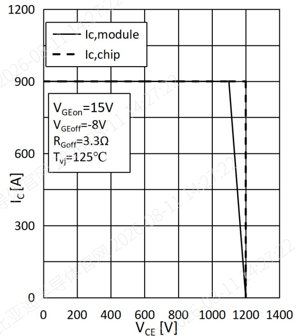
Fig. 8 Reverse Bias safe operating area
