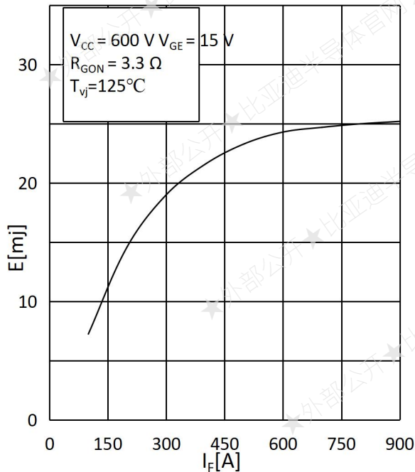
Fig.7 Reverse recovery Energy
