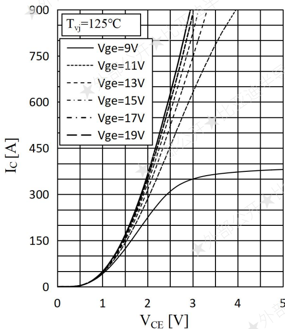
Fig.3 Output Characteristics
