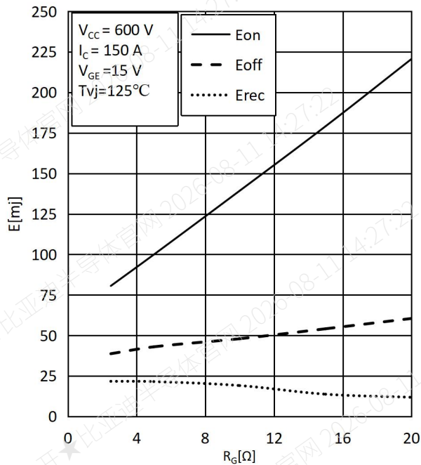
Fig.5 Switching Loss vs. Gate Resistor
