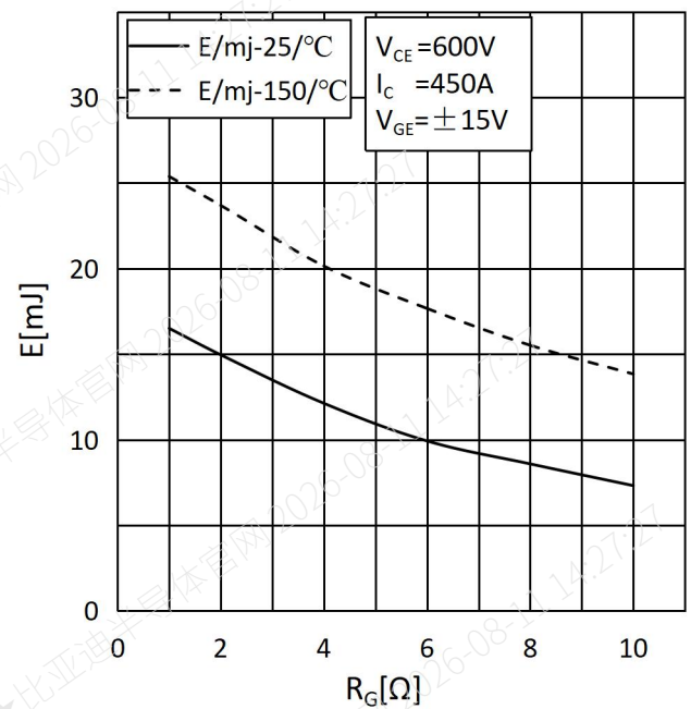
图 8: 反向恢复损耗与门极电阻关系 Fig.8 Reverse recovery Energy vs. Gate Resistor
