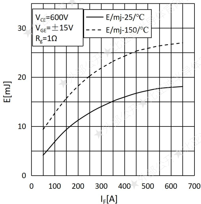
图 7 反向恢复损耗 Fig.7 Reverse recovery Energy
