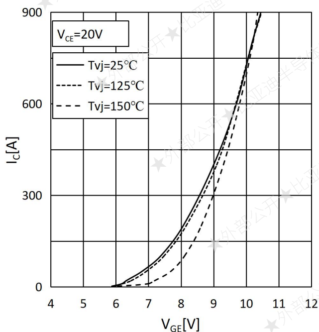
Fig.3: Transfer Characteristics
