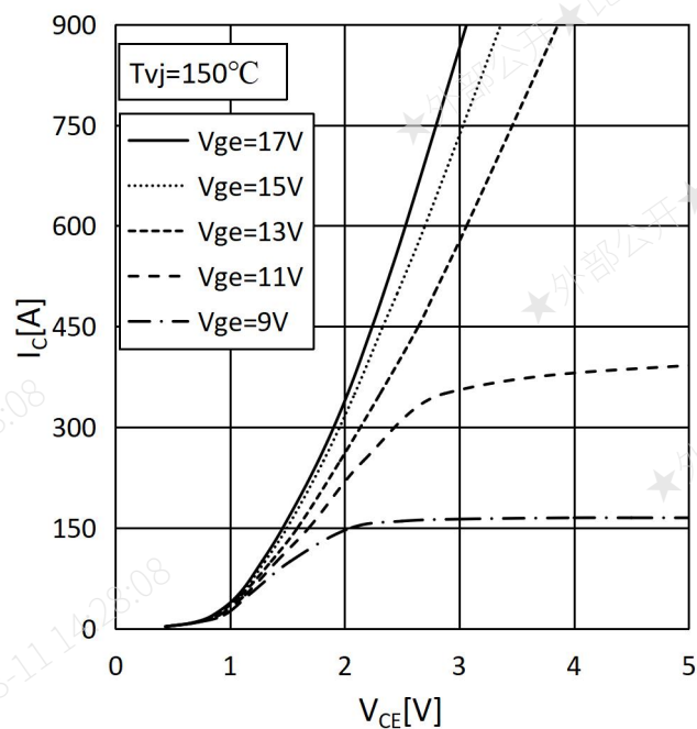
Fig.2: Output characteristics
