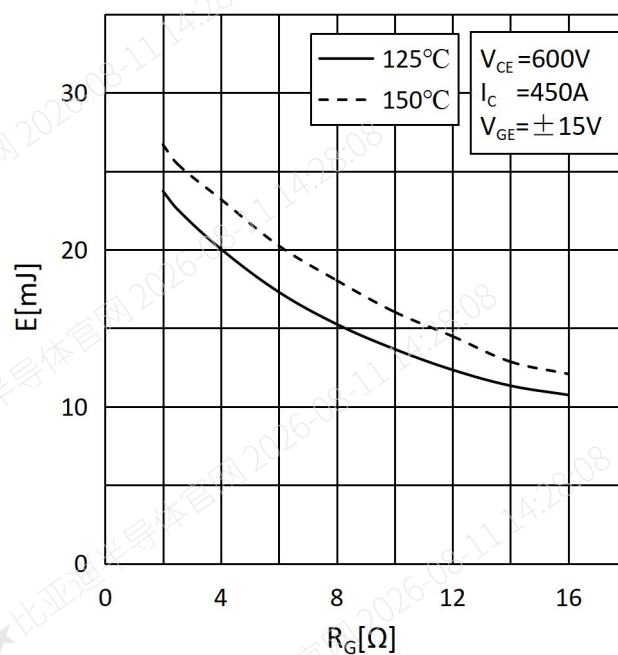
Fig.8: Reverse recovery Energy vs. Gate Resistor
