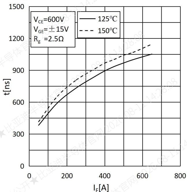
Fig.9: Reverse Recovery Times vs. IF
