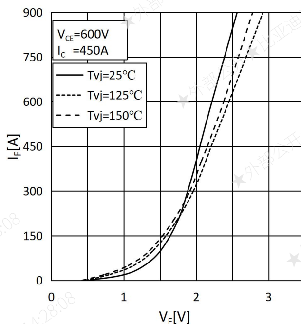
Fig.6: Forward characteristic
