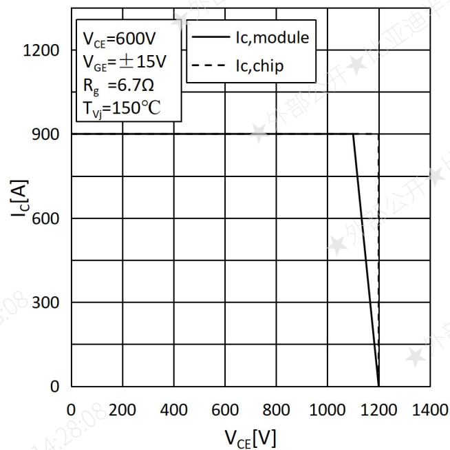
Fig.10: Reverse Bias Safe Operating Area
