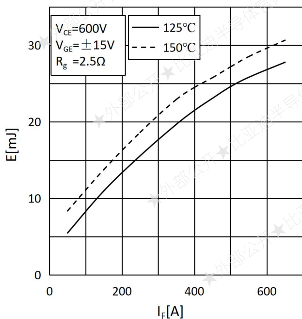
Fig.7: Reverse recovery Energy
