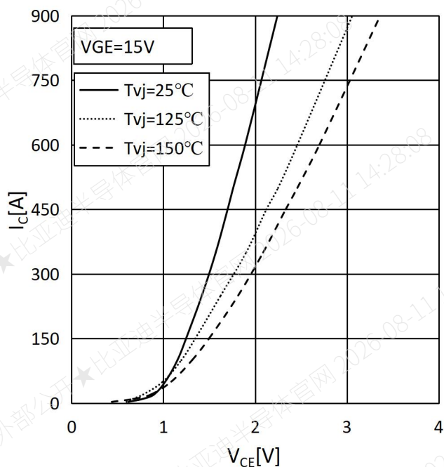
Fig.1 Output Characteristics
