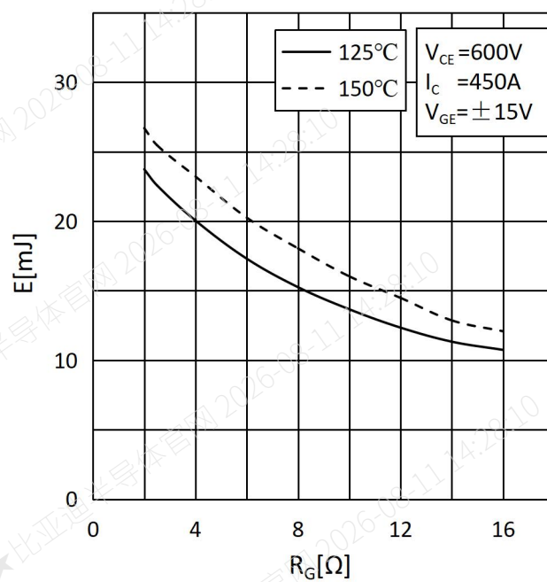
Fig.8: Reverse recovery Energy vs. Gate Resistor
