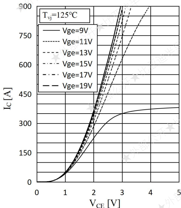
Fig.3 Output Characteristics
