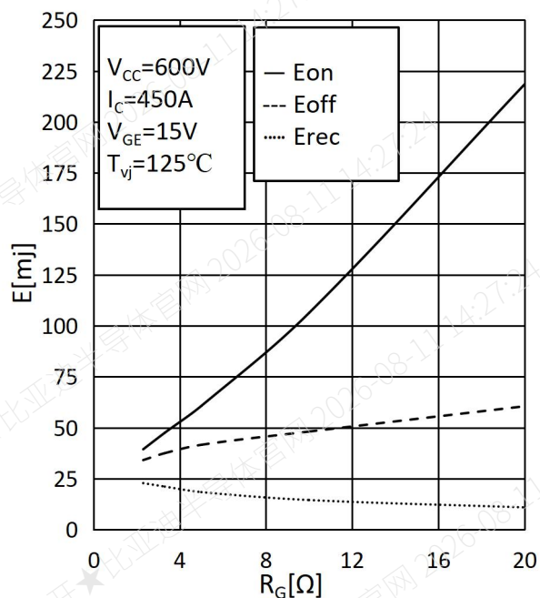
Fig.5 Switching Loss vs. Gate Resistor
