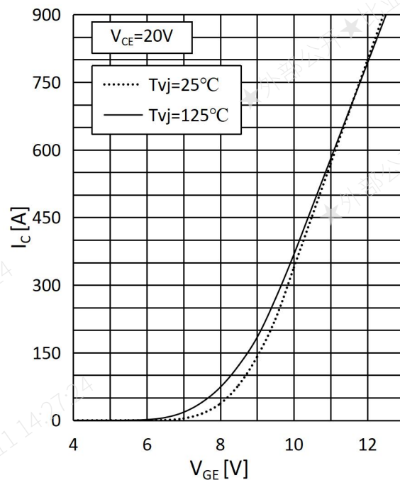
Fig.2 Transfer Characteristics
