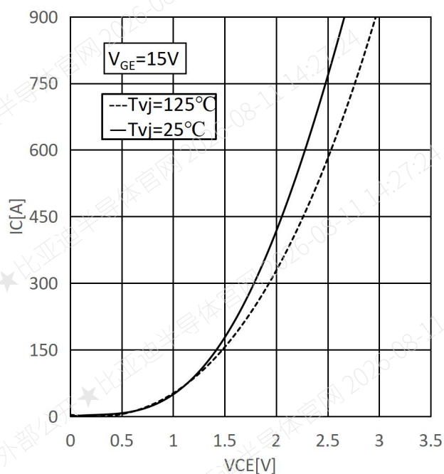
Fig.1 Output Characteristics
