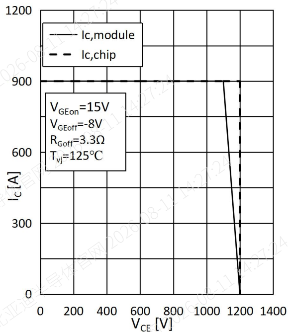
Fig. 8 Reverse Bias safe operating area
