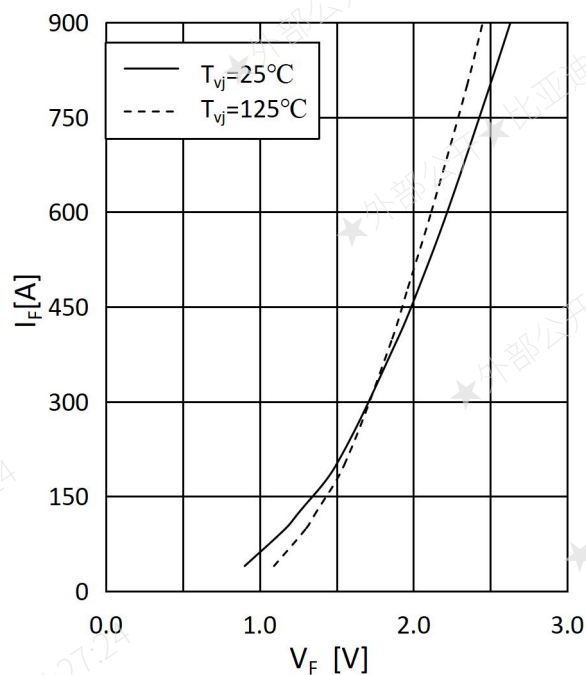
Fig.6 Forward Characteristics
