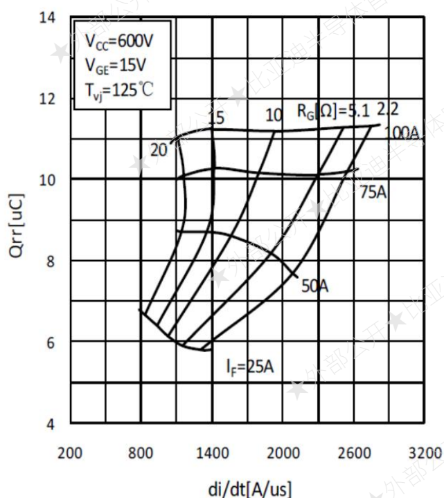
Fig.11 Typ. FRD Recovery Charge
