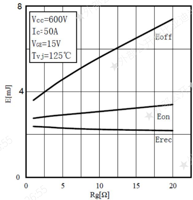
Fig.6 Switching Loss vs. Gate Resistor
