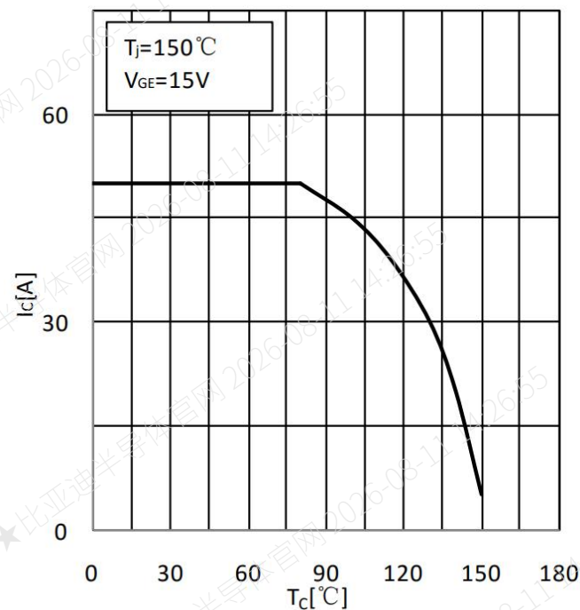
Fig. 12 Rate Current vs. Temperature ( T_c )
