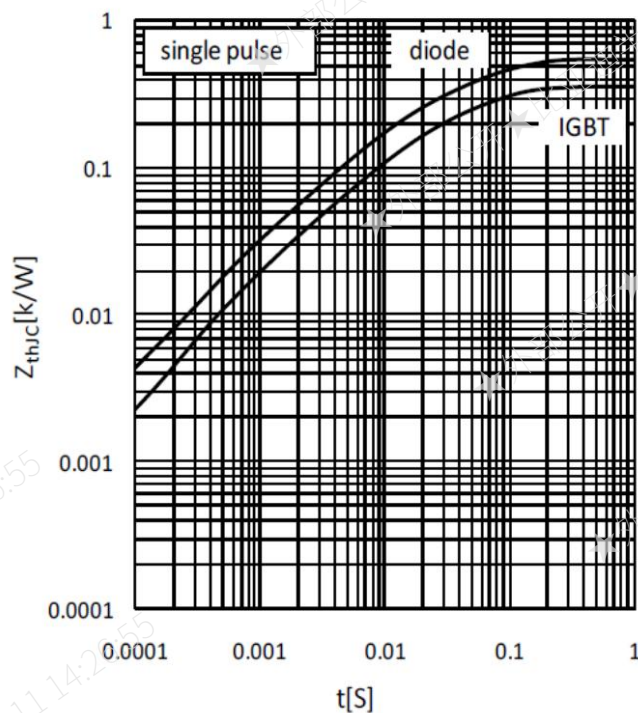
Fig.14 Typ. Transient Thermal Impedance
