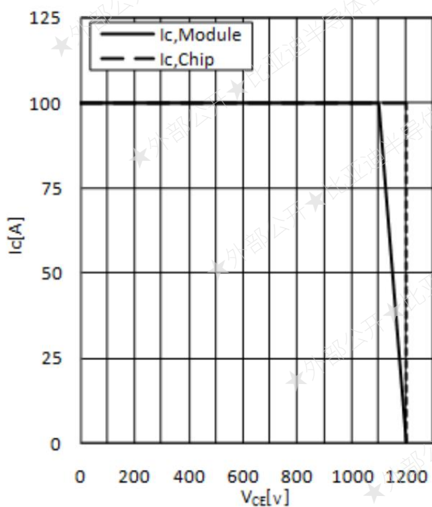
Fig.15 Reverse Bias Safe Operating Area (RBSOA)
