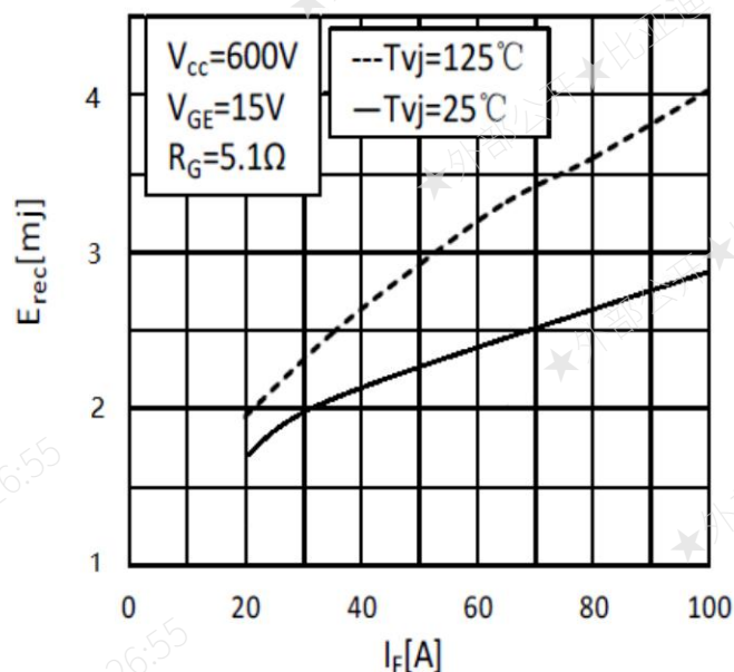
Fig.10 Typ. Switching Losses Diode-Inverter
