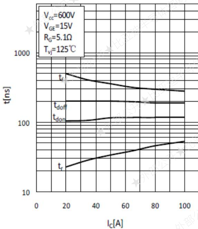
Fig.7 Typ. Switching Times vs. IC
