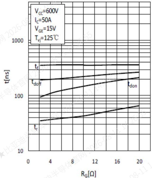
Fig.8 Typ. Switching Times vs. Gate Resistor
