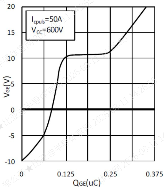
Fig.13 Typ. Gate Charge Characteristics
