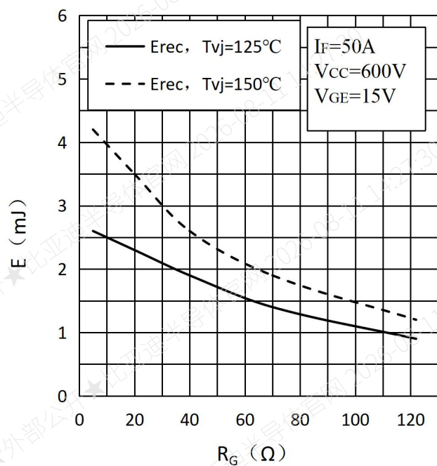
Fig.9 Switching Loss of Diode vs. Gate Resistor
