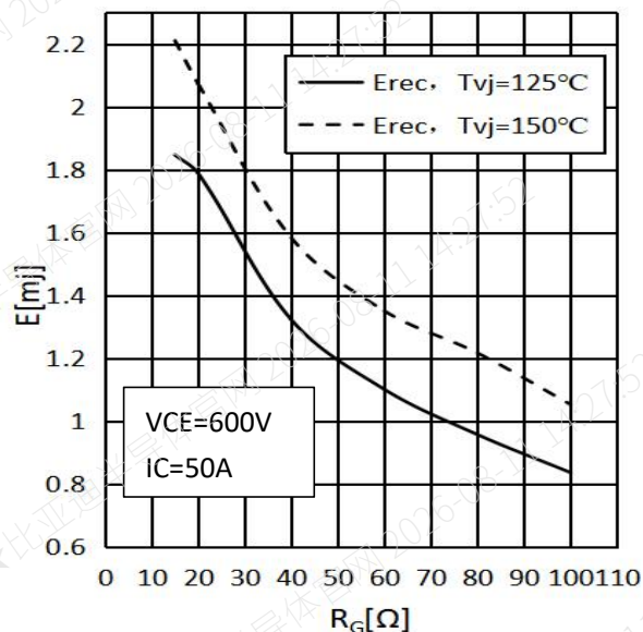
Fig.8 Reverse recovery Energy vs. Gate Resistor
