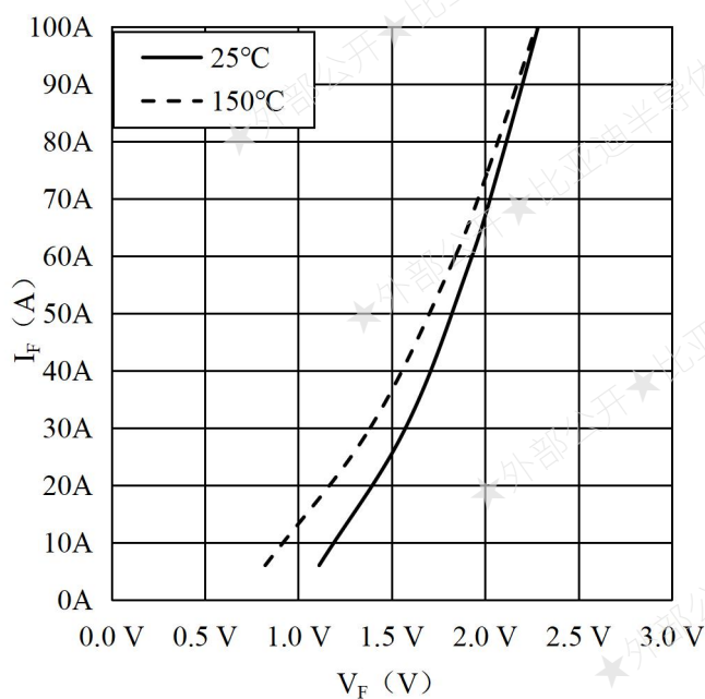
Fig.7 Typ. Forward Characteristics of Diode-Inverter 图 7 二极管正向偏压特性-逆变器
