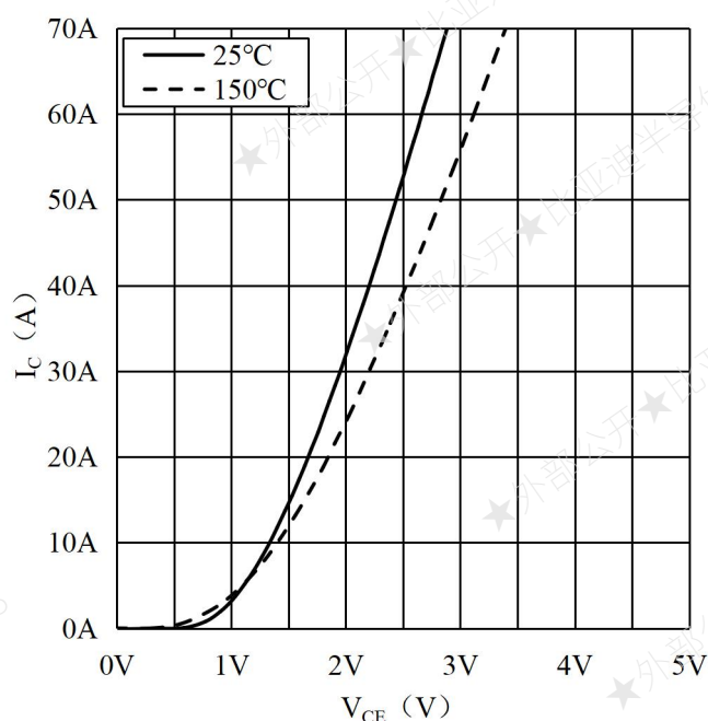
Fig.11 Typ. Output Characteristics, Brake-Chopper
