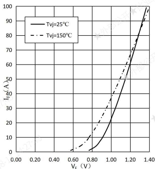
Fig.10 Forward Characteristics of Diode-Rectifier
