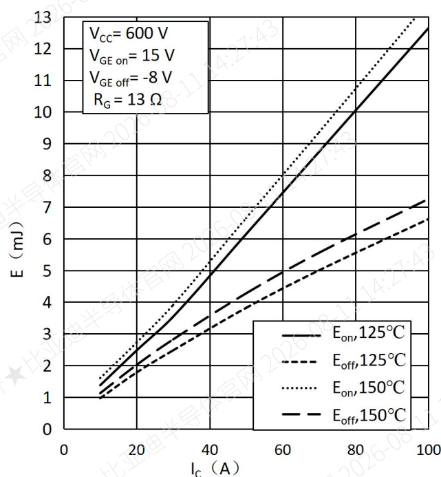
Fig.4 Switching Loss vs. Collector Current-Inverter
