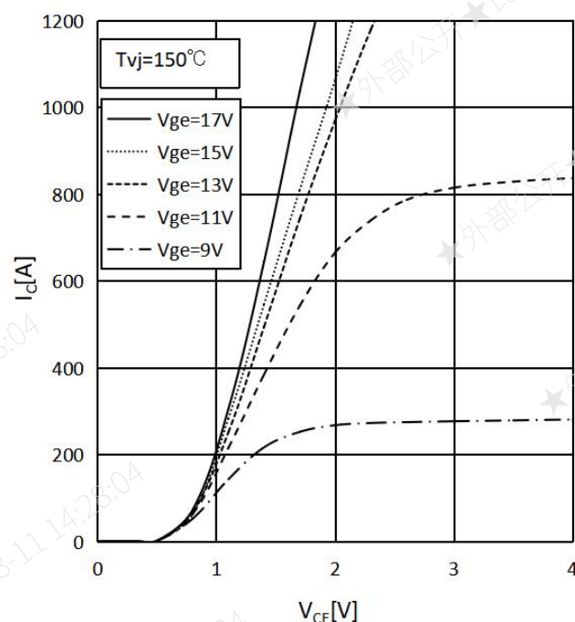
Fig.2: Output characteristics
