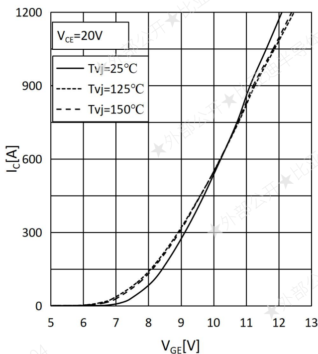
Fig.3: Transfer Characteristics
