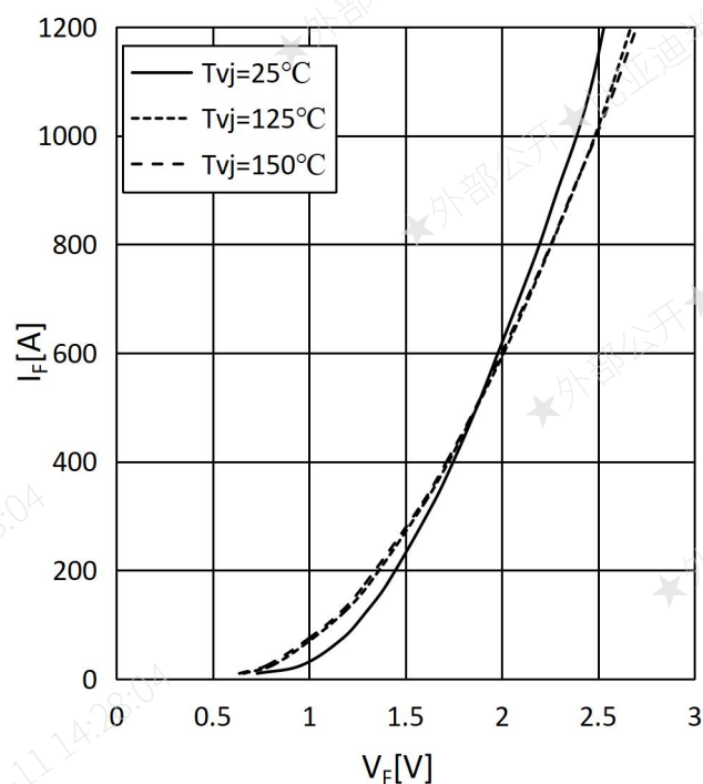
Fig.6: Forward characteristic
