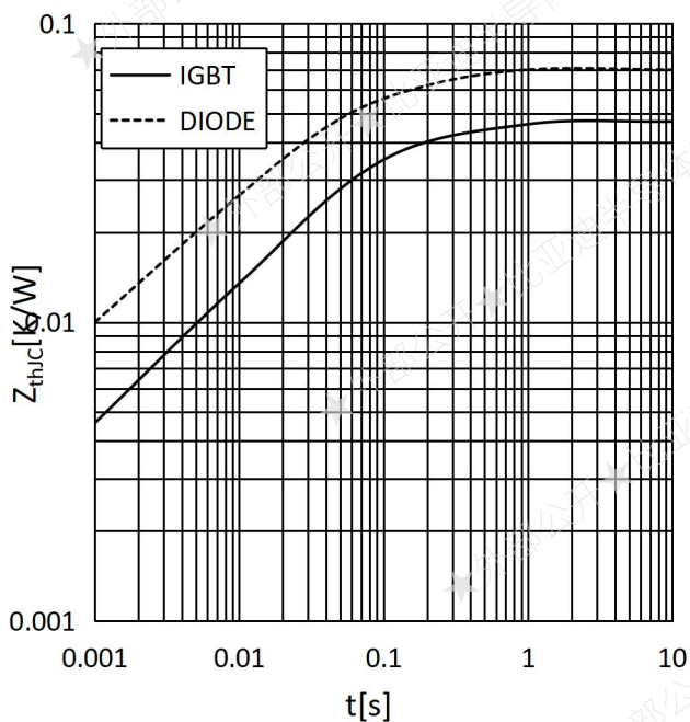
Fig.11: Typ. transient thermal impedance ZthJC
