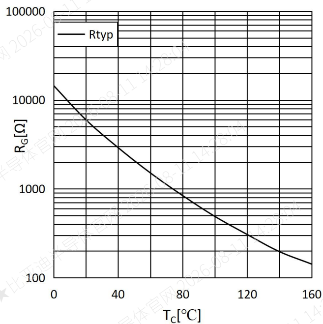
Fig.12: Typ. NTC-Temperature Characteristics
