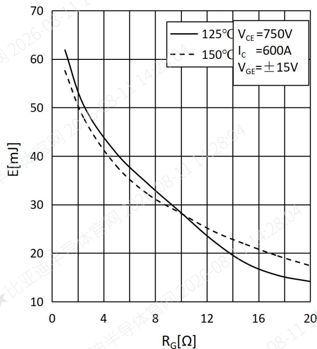
Fig.8: Reverse recovery Energy vs. Gate Resistor
