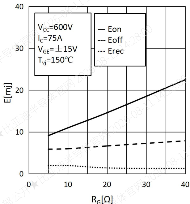
图 5 开关损耗和门极电阻 Fig.5 Switching Loss vs. Gate Resistor
