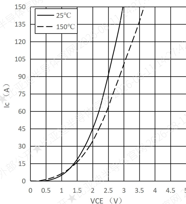
Fig.1 Typ. Output Characteristics-Inverter
