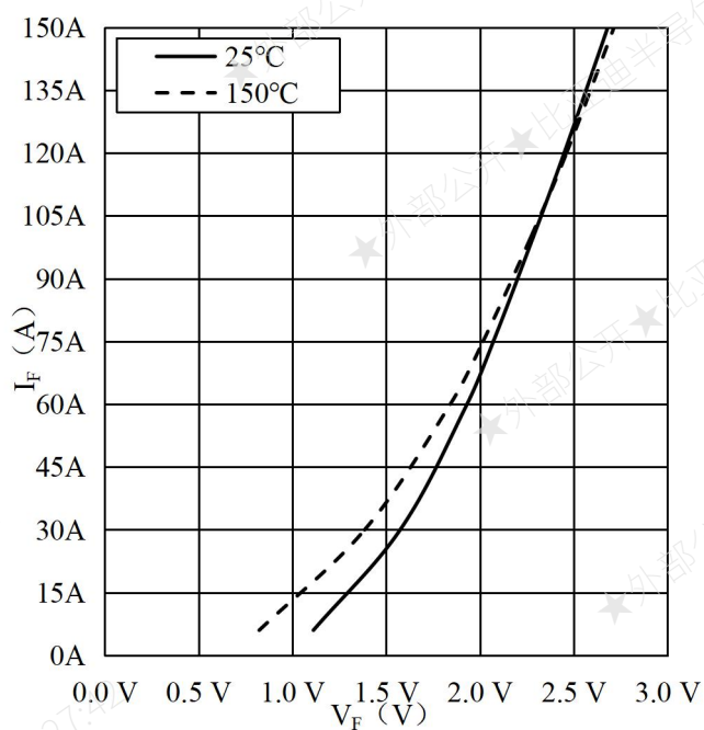
Fig.7 Typ. Forward Characteristics of Diode-Inverter 图 7 二极管正向偏压特性-逆变器
