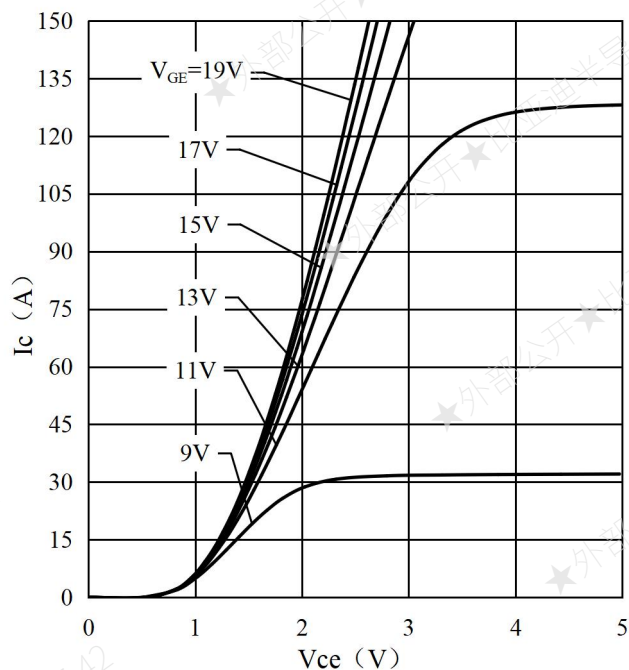
Fig.3 Typ. Output Characteristics-Inverter
