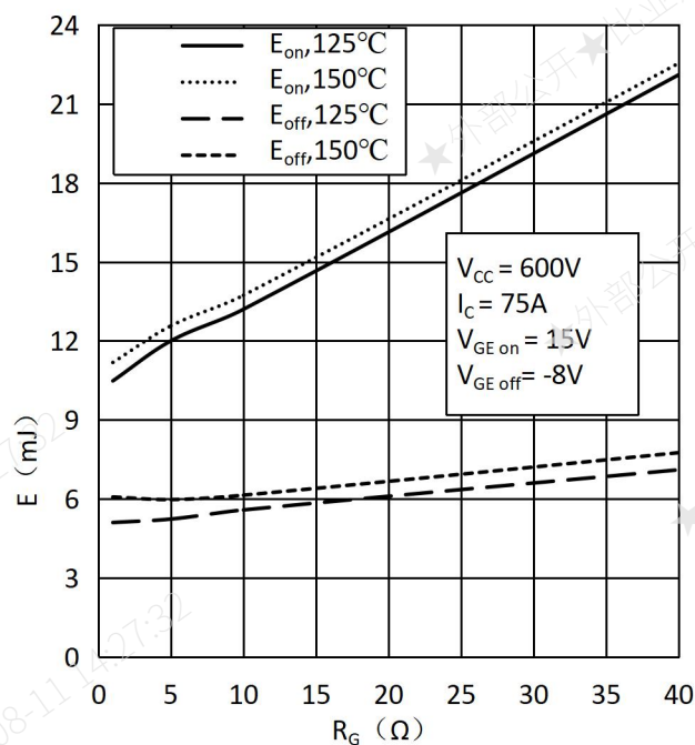
Fig.6 Switching Loss of IGBT vs. Gate Resistor -
