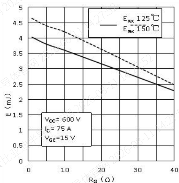
Fig.8 Reverse recovery Energy vs. Gate Resistor
