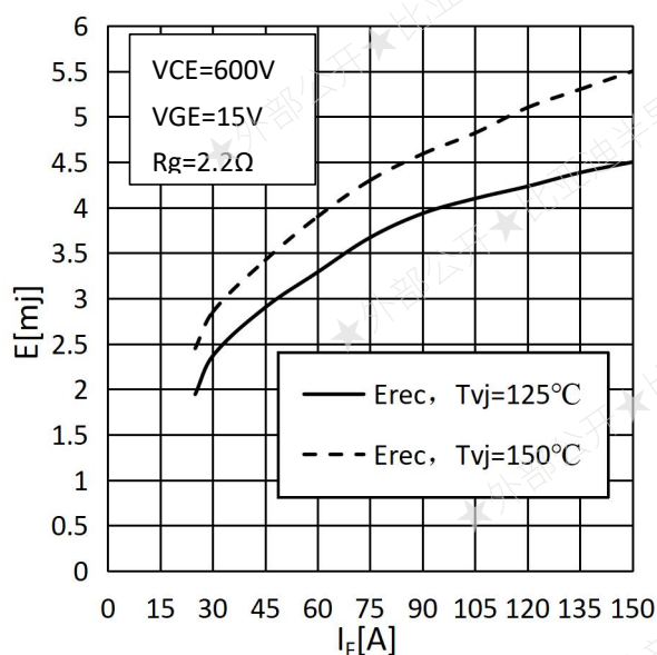
Fig.7 Reverse recovery Energy
