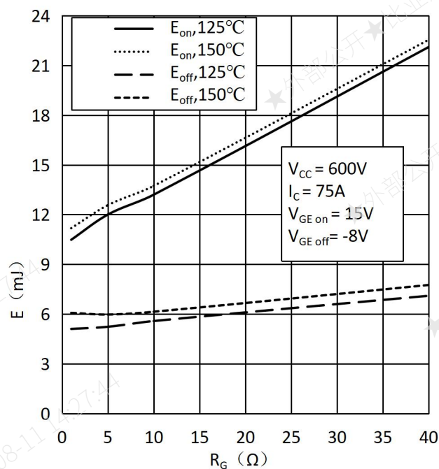
Fig.6 Switching Loss of IGBT vs. Gate Resistor -
