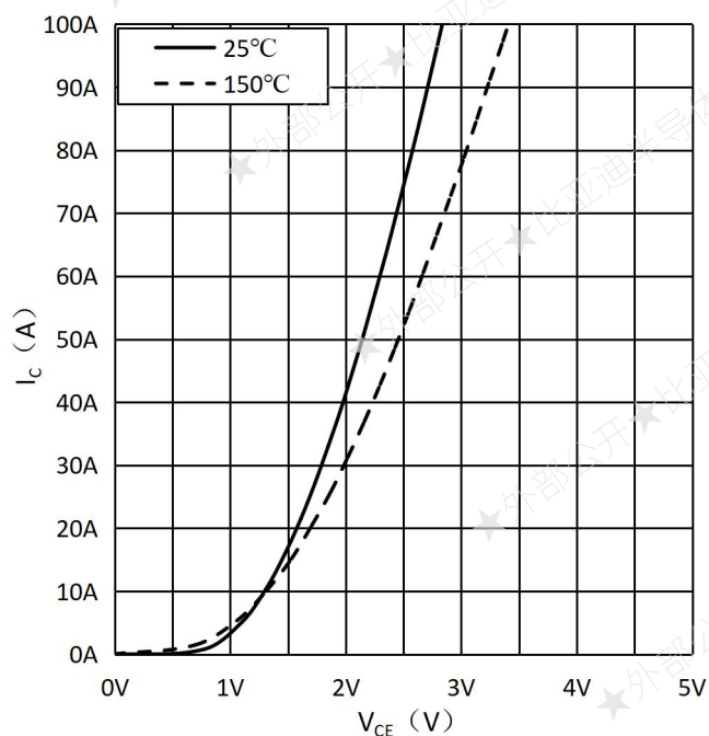
Fig.11 Typ. Output Characteristics, Brake-Chopper
