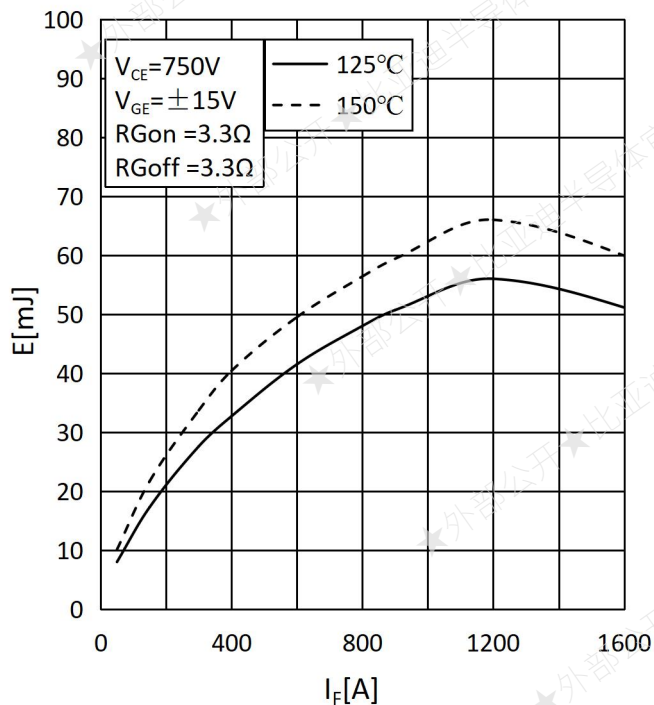
Fig.7: Reverse recovery Energy
