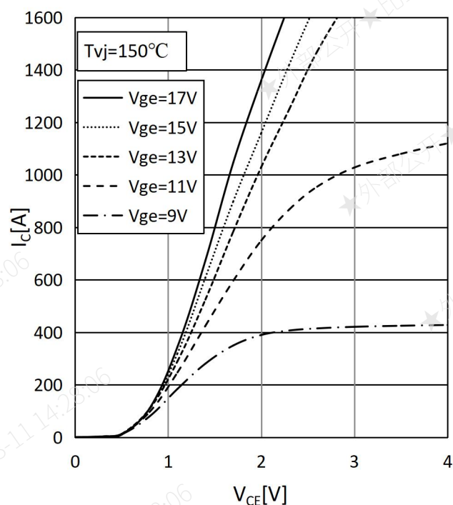
Fig.2: Output characteristics
