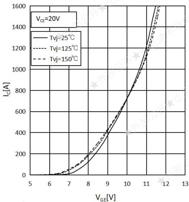
Fig.3: Transfer Characteristics
