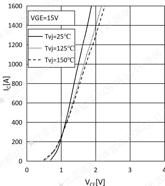
Fig.1 Output Characteristics
