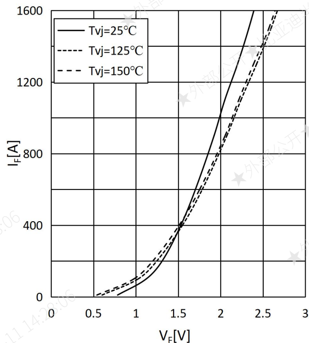
Fig.6: Forward characteristic
