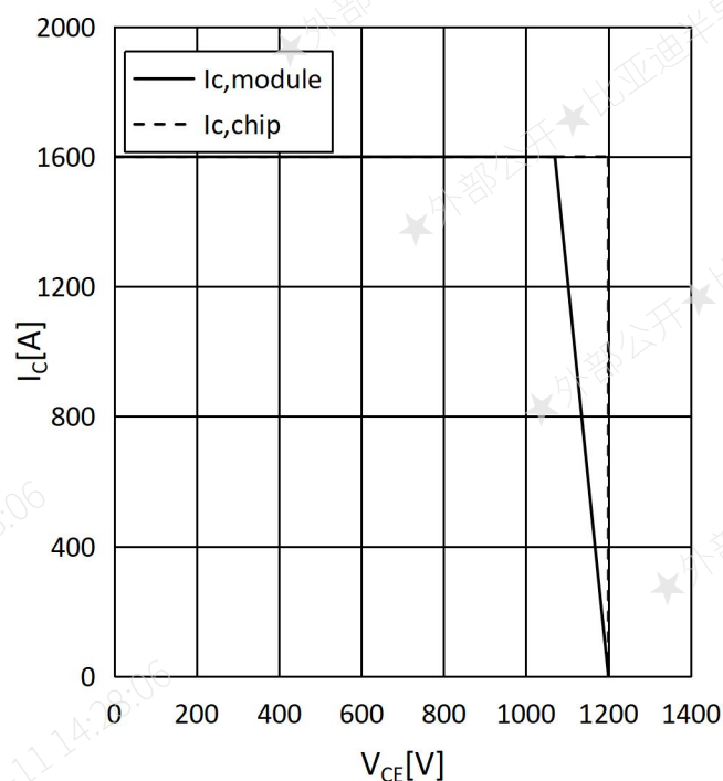
Fig.10: Reverse Bias Safe Operating Area
