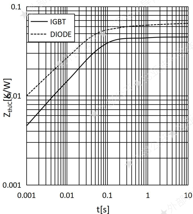
Fig.11: Typ. transient thermal impedance ZthJC
