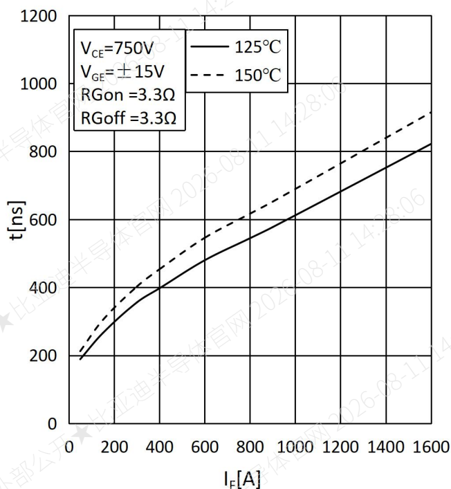
Fig.9: Reverse Recovery Times vs. IF
