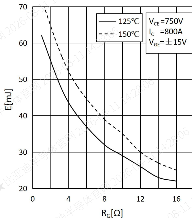
Fig.8: Reverse recovery Energy vs. Gate Resistor
