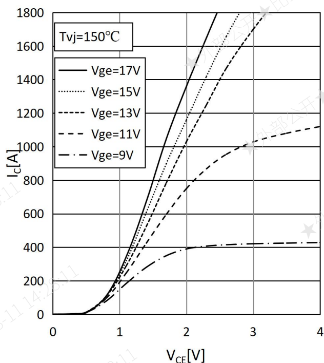
Fig.2: Output characteristics
