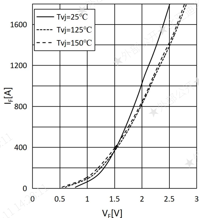
Fig.6: Forward characteristic
