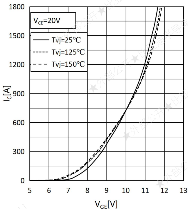
Fig.3: Transfer Characteristics
