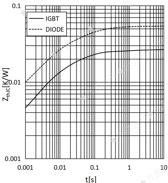
Fig.11: Typ. transient thermal impedance ZthJC
