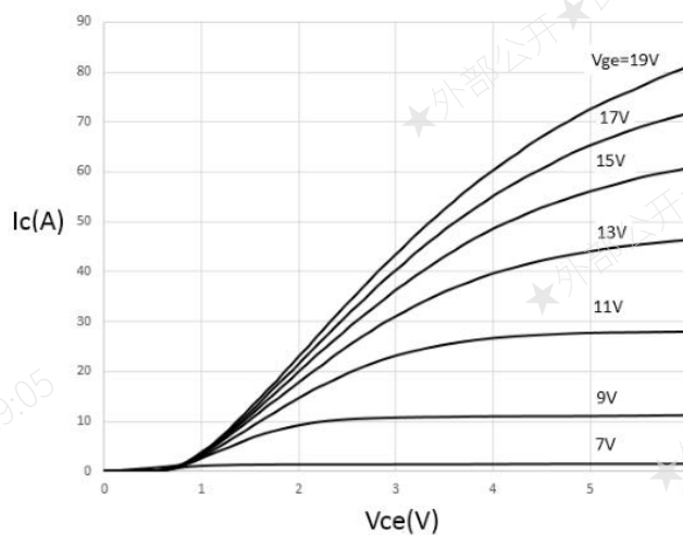
Figure 2. Typical output characteristic( T_j=150^{\circ}\text{C} )
