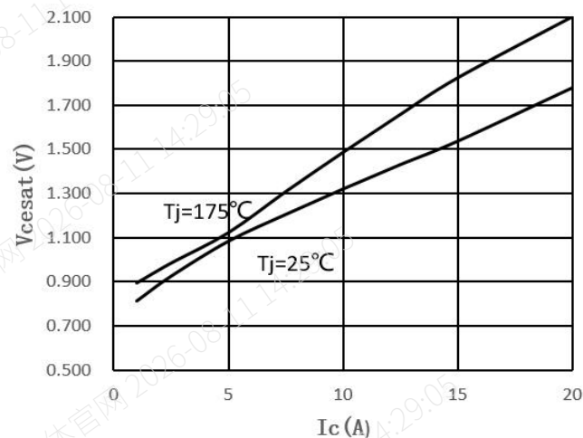
Figure 4. V_{\text{cesat}} vs. I_c
