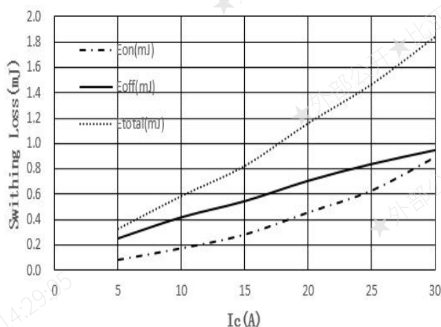
Figure 8. Switching energy losses vs I_c ( T_j=150^\circ\text{C} , V_{CE}=400\text{V} , V_{GE}=15\text{V} , R_g=10\ \Omega )
