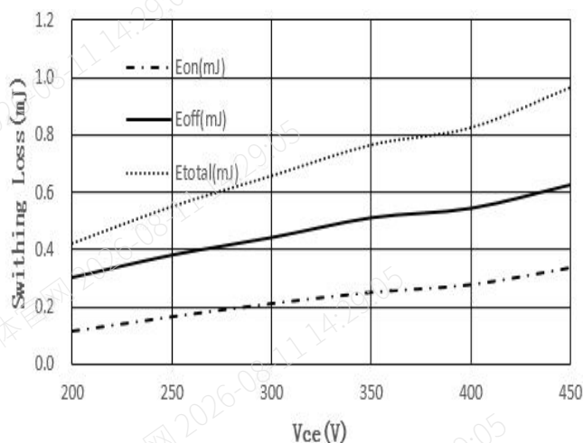
Figure 10. Switching energy losses vs V_{CE} ( T_j=150^\circ\text{C} , V_{GE}=15\text{V} , I_C=15\text{A} , R_g=10\ \Omega )
