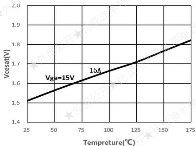
Figure 3. V_{\text{cesat}} vs. T_j
