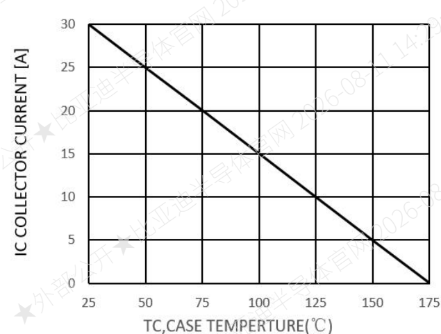
Figure 12. I_c vs T_c
