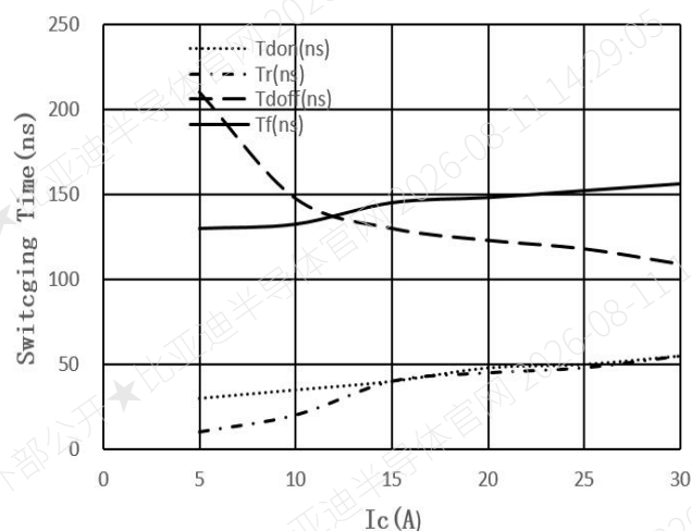
Figure 6. Switching times vs I_c ( T_j=150^{\circ}\text{C} , V_{\text{GE}}=15\text{V} , V_{\text{CE}}=400\text{V} , R_g=10\Omega )
