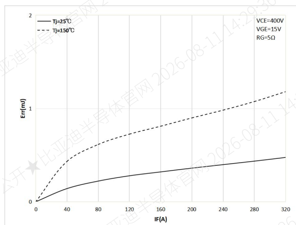
Figure 18. Reverse Recovery Energy Loss vs. Collector Current
