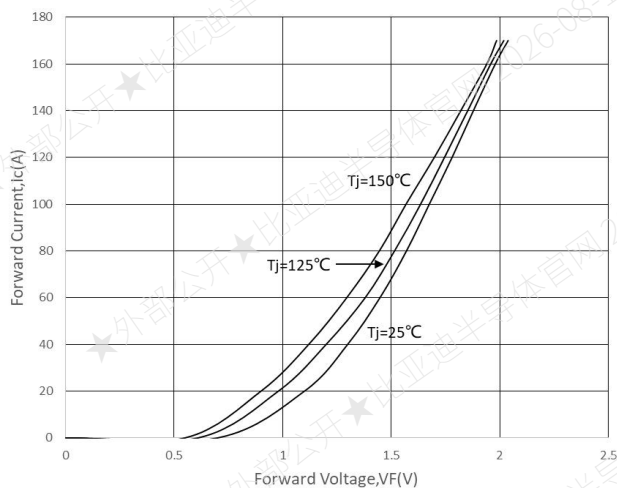
Figure 15. Forward Characteristics
