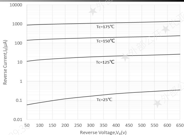
Figure 20. Reverse Current
