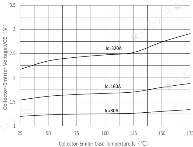
Figure 5. Saturation Voltage vs. Case Temperature at Variant Current Level( V_{GE}=15\text{V} )
