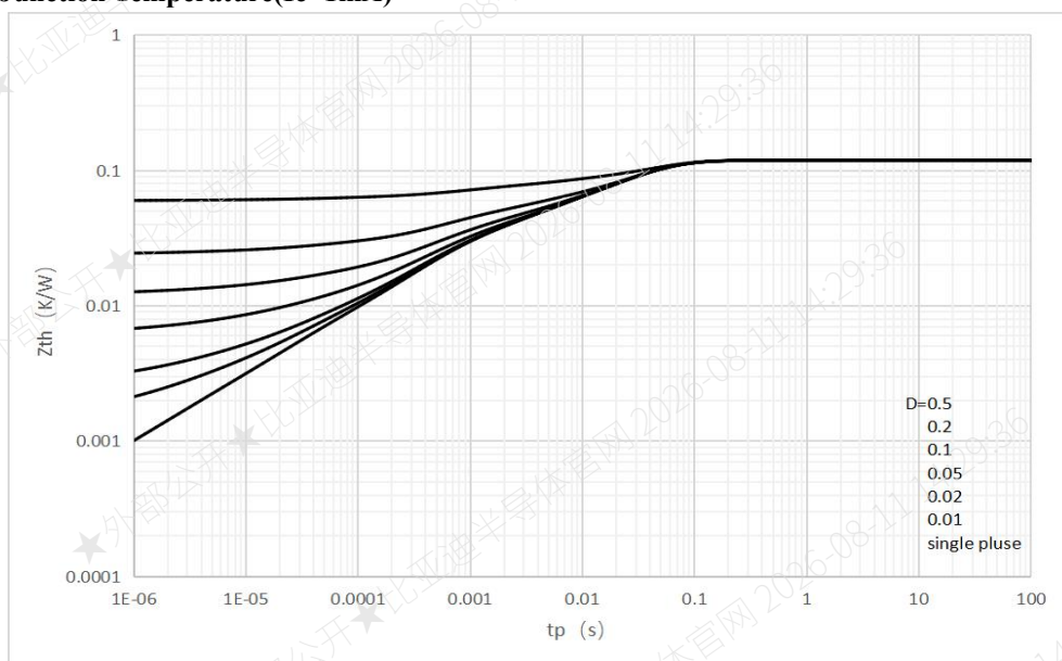
Figure 21. Transient Thermal Impedance of IGBT
