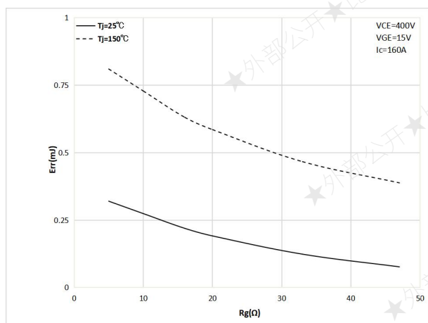
Figure 17. Reverse Recovery Energy Loss vs. Gate Resistance
