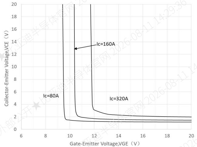
Figure 6. Saturation Voltage vs. V_{GE} ( T_j=25^{\circ}\text{C} )
