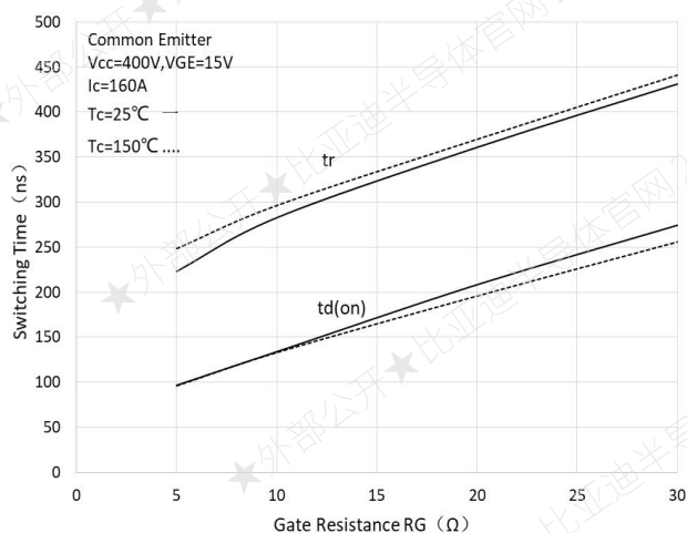
Figure 9. Turn-on Characteristics vs. Gate Resistance
