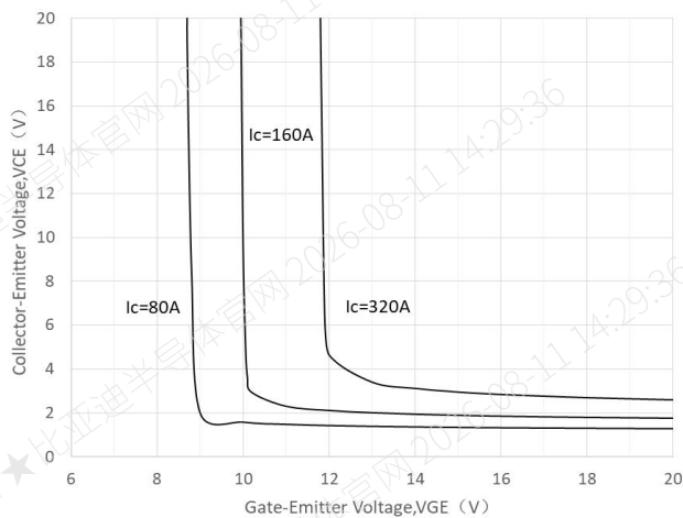
Figure 7. Saturation Voltage vs. V_{GE} ( T_j=150^\circ\text{C} )
