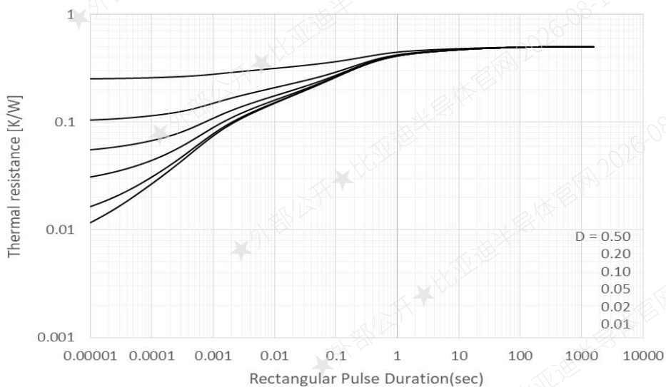
Figure 15. Transient Thermal Impedance of Diode
