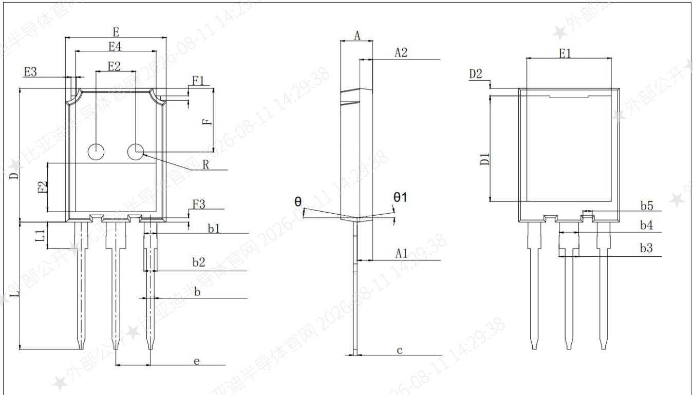
Common Dimensions (Units:Millimeter)
