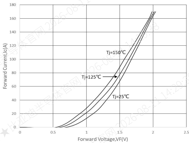
Figure 7. Forward Characteristics
