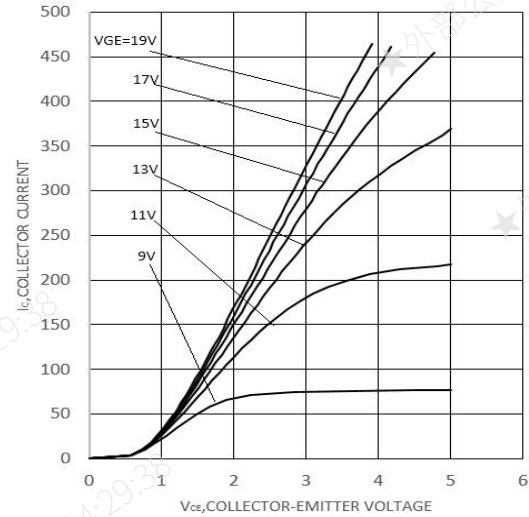
Figure 2. Typical output characteristic( T_j=150^{\circ}\text{C} )
