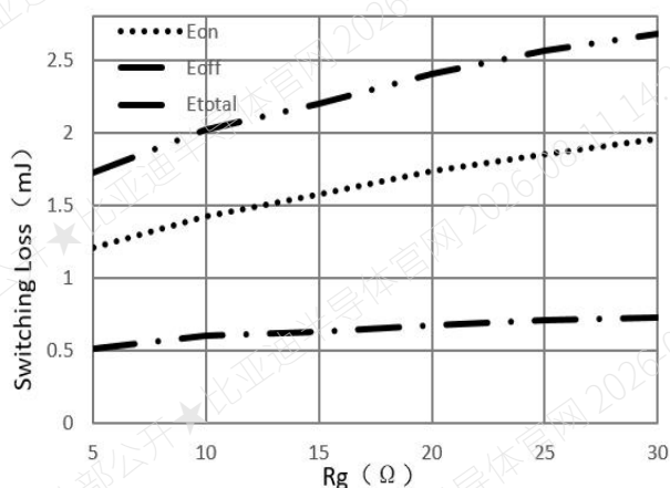
Figure 12. Switching energy losses vs R_g ( T_j=150^\circ C, V_{CE}=400V, V_{GE}=15V, I_C=30A )
