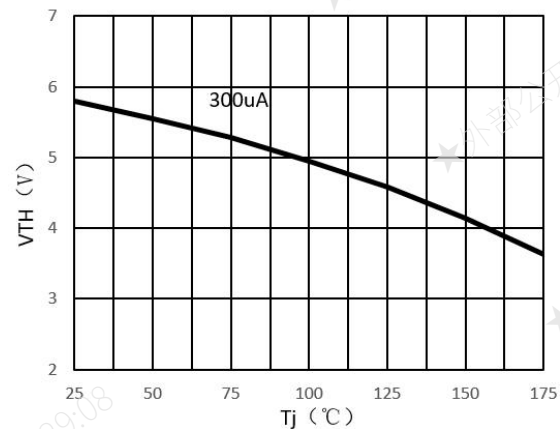
Figure 5. V_{TH} vs. T_j
