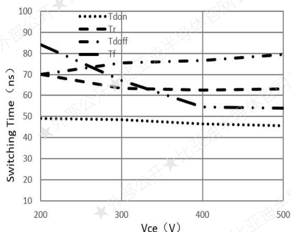
Figure 9. Switching times vs V_{CE} ( T_j=150^\circ C, V_{GE}=15V, I_C=30A, R_G=10\Omega )
