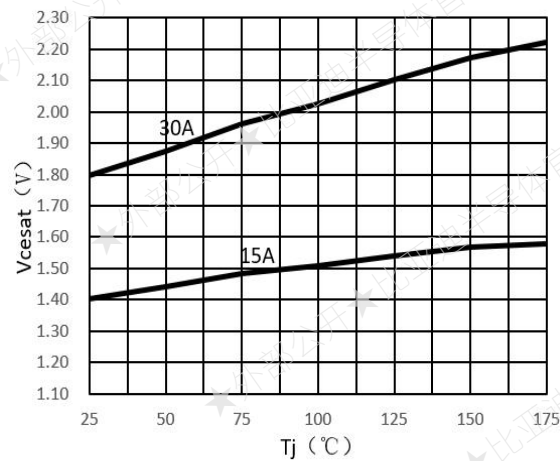
Figure 3. V_{cesat} vs. T_j
