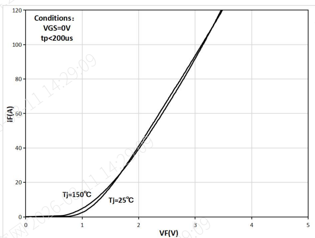
Figure 10. Typical diode forward current as a function of forward voltage
