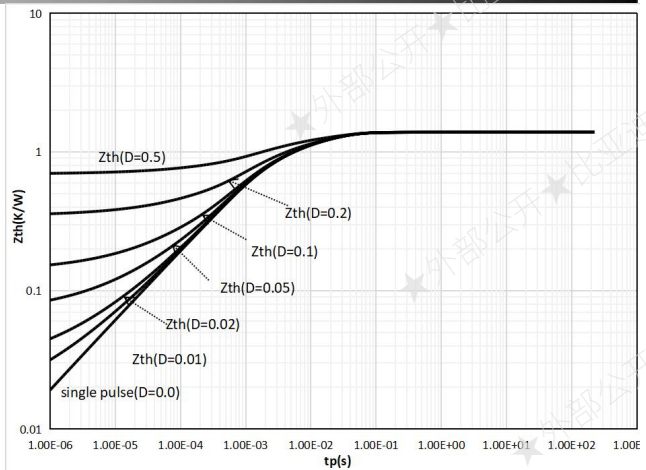
Figure 14.Diode Transient thermal impedance as a function of pulse width( D=t_p/T )
