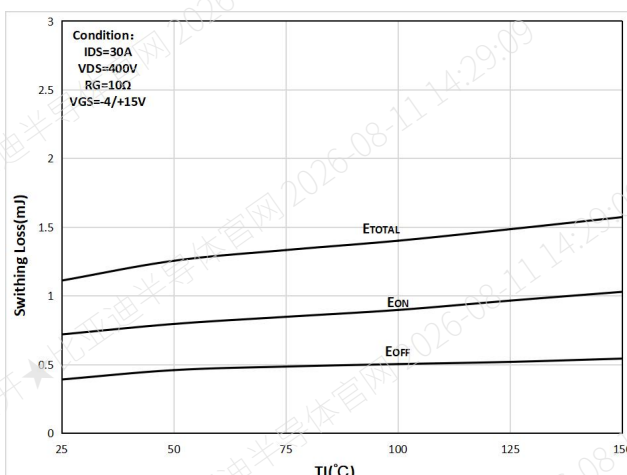
Figure 12. Typical switching energy losses as a function of junction temperature ( V_{CE}=400V, I_C=30A, V_{GE}=15V, R_G=10\Omega )
