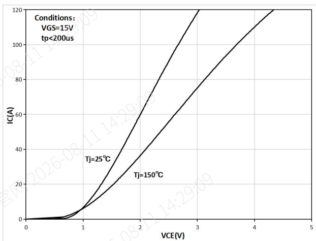
Figure 4. Typical collector current as a function of collector-emitter saturation voltage ( V_{GE}=15\text{V} )
