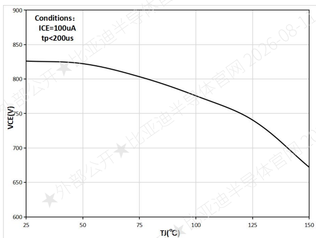
Figure 9. Collector-Emitter breakdown voltage as a function junction temperature ( I_C=100uA )
