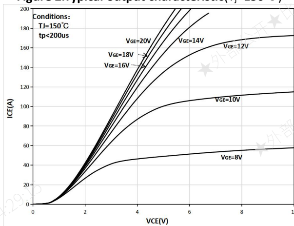
Figure 4. Typical collector current as a function of collector-emitter saturation voltage
