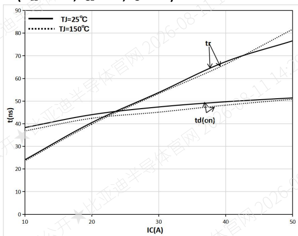
Figure 12. Typical turn-on characteristic as a function of collector current ( V_{CE}=400V, V_{GE}=15V, R_G=10\Omega )
