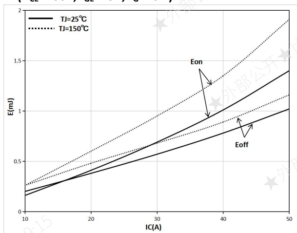
Figure 11. Typical switching energy losses as a function of collector current ( V_{CE}=400V, V_{GE}=15V, R_G=10\Omega )
