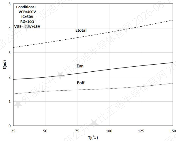
Figure 15. Typical switching energy losses as a function of junction temperature
