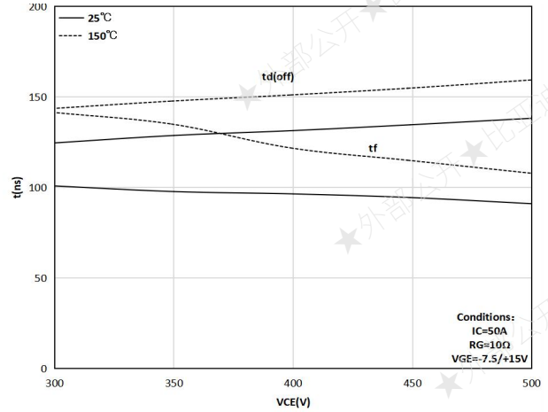
Figure 14. Typical turn-off characteristic as a function of collector emitter voltage
