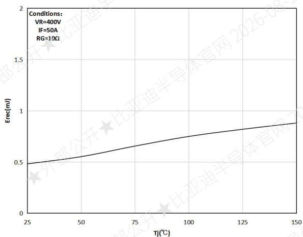
Figure 21. Typical reverse energy losses as a function of junction temperature
