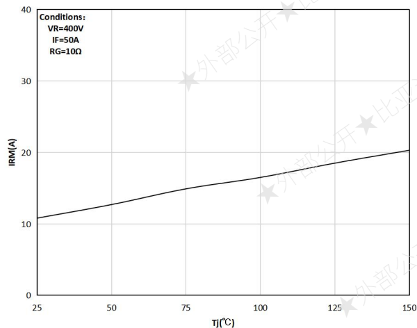
Figure 20. Typical reverse recovery current as a function of junction temperature
