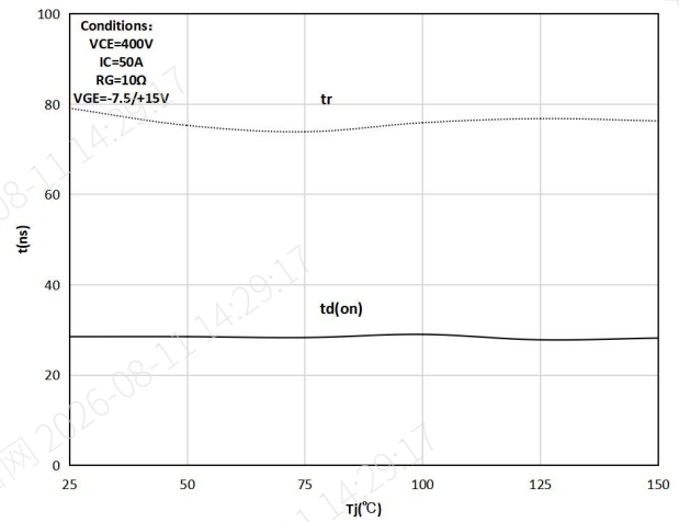
Figure 16. Typical turn-on characteristic as a function of junction temperature
