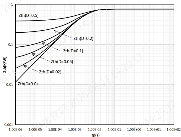
Figure 25. Diode Transient thermal impedance as a function of pulse width ( D = t_p / T )
