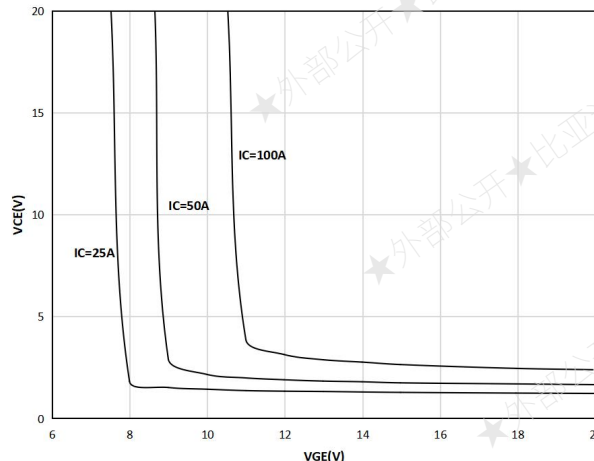
Figure 8. Typical turn-on characteristic as a function of collector current
