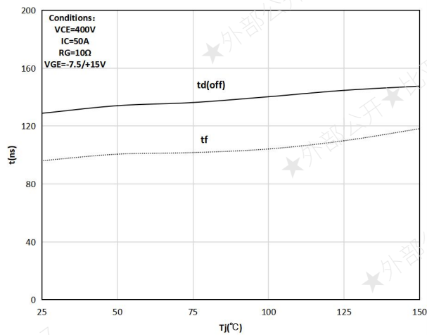
Figure 17. Typical turn-off characteristic as a function of junction temperature
