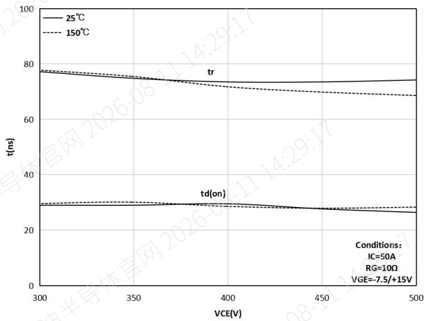
Figure 13. Typical turn-on characteristic as a function of collector emitter voltage
