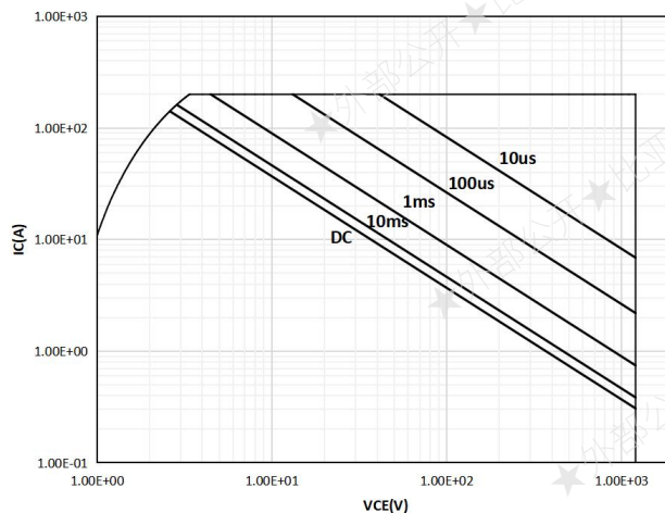
Figure 26. Forward bias safe operating area ( D=0, T_c=25^\circ\text{C}, T_j \leq 150^\circ\text{C}, V_{GE}=15\text{V}, I_{Cmax} defined by design - not subject to production test)
