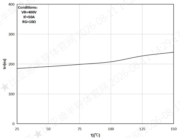
Figure 18. Typical reverse recovery time as a function of junction temperature
