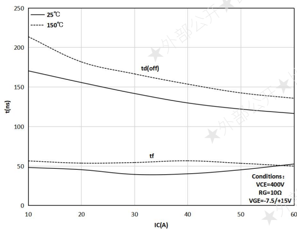
Figure 11. Typical turn-off characteristic as a function of collector current
