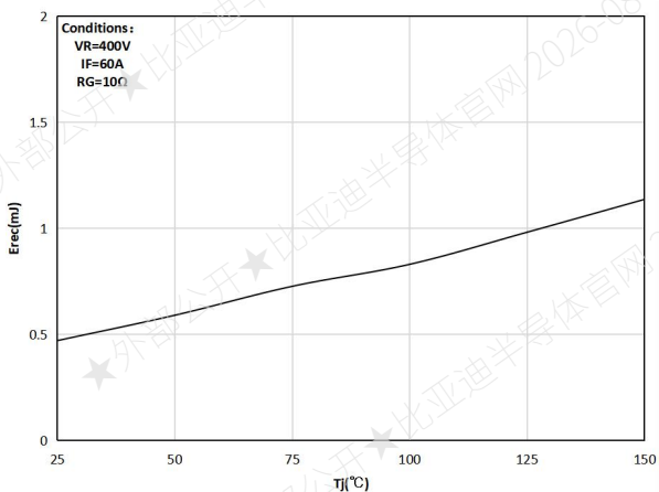
Figure 21. Typical reverse energy losses as a function of junction temperature
