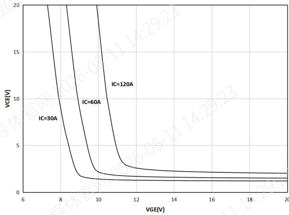
Figure 7. Typical collector-emitter saturation voltage as a function of gate-emitter voltage ( T_j=25^\circ\text{C} )
