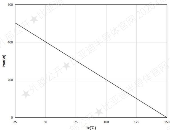
Figure 27. Power dissipation as a function of case temperature ( T_j \leq 150^\circ\text{C} )
