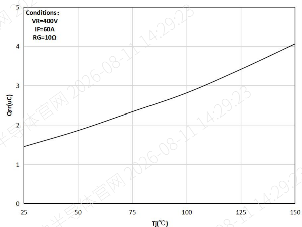
Figure 19. Typical reverse recovery charge as a function of junction temperature
