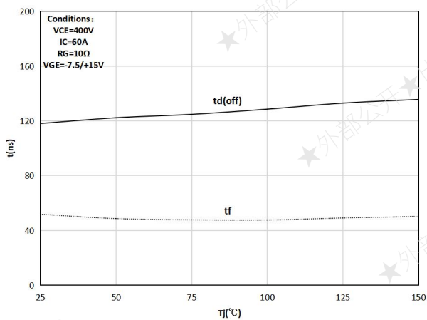
Figure 17. Typical turn-off characteristic as a function of junction temperature
