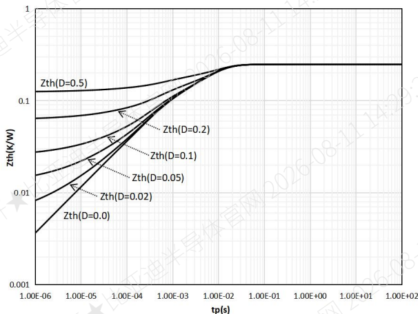
Figure 24. IGBT Transient thermal impedance as a function of pulse width( D=t_p/T )
