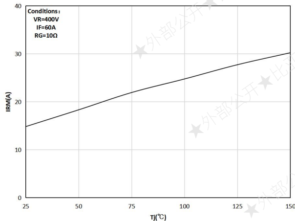
Figure 20. Typical reverse recovery current as a function of junction temperature
