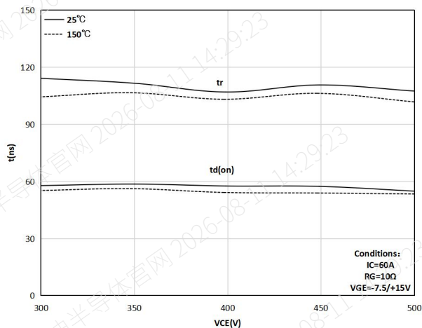
Figure 13. Typical turn-on characteristic as a function of collector emitter voltage
