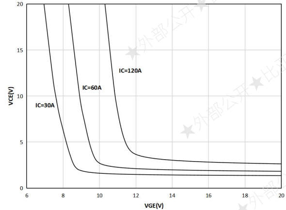
Figure 8. Typical collector-emitter saturation voltage as a function of gate-emitter voltage ( T_j=150^\circ\text{C} )
