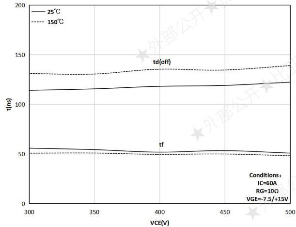
Figure 14. Typical turn-off characteristic as a function of collector emitter voltage
