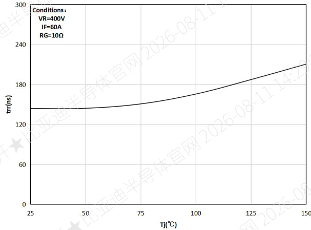
Figure 18. Typical reverse recovery time as a function of junction temperature
