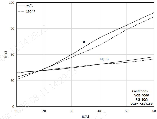
Figure 10. Typical turn-on characteristic as a function of collector current
