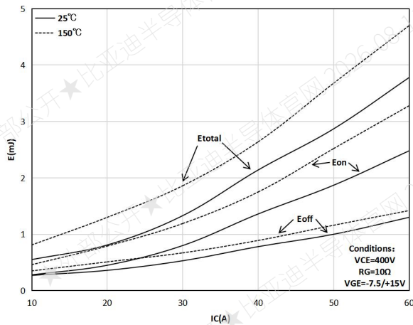
Figure 9. Typical switching energy losses as a function of collector current
