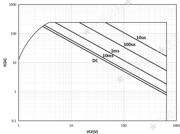
Figure 26. Forward bias safe operating area ( D=0, T_c=25^\circ\text{C}, T_j \leq 150^\circ\text{C}, V_{GE}=15\text{V}, I_{Cmax} defined by design - not subject to production test)
