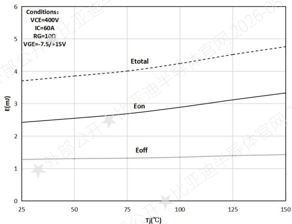
Figure 15. Typical switching energy losses as a function of junction temperature
