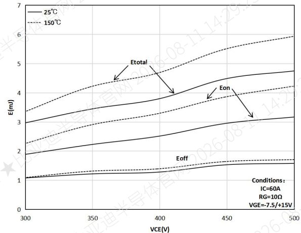
Figure 12. Typical switching energy losses as a function of collector emitter voltage
