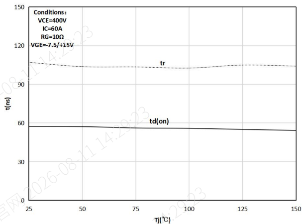
Figure 16. Typical turn-on characteristic as a function of junction temperature
