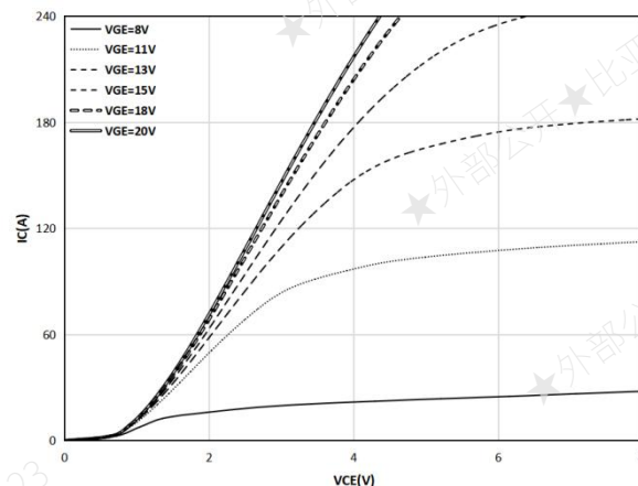
Figure 2. Typical output characteristic ( T_j=150^{\circ}\text{C} )
