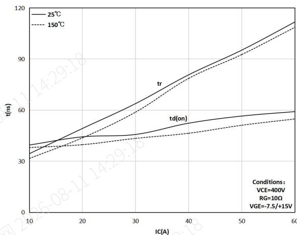
Figure 10. Typical turn-on characteristic as a function of collector current
