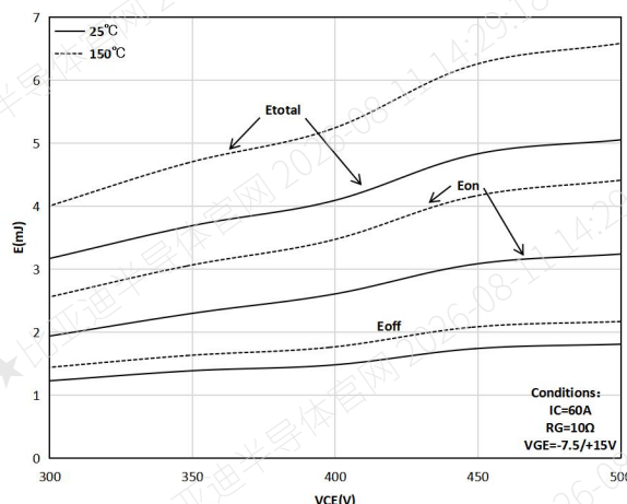
Figure 12. Typical switching energy losses as a function of collector emitter voltage
