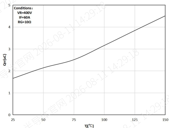
Figure 19. Typical reverse recovery charge as a function of junction temperature
