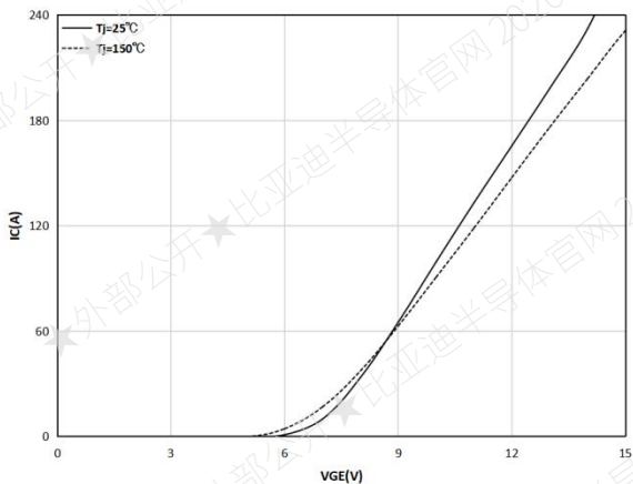
Figure 3. Typical transfer characteristic ( V_{ce}=20\text{V} )
