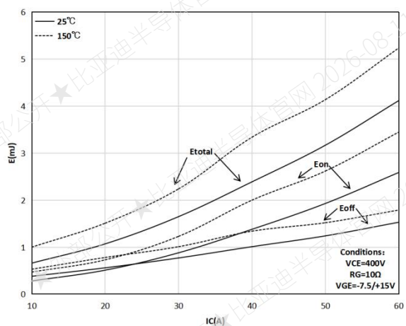
Figure 9. Typical switching energy losses as a function of collector current
