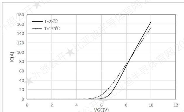
Figure 3. Typical transfer characteristic ( V_{CE}=60\text{V} )
