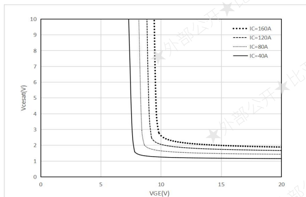
Figure 5. Typical collector-emitter saturation voltage as a function of gate-emitter voltage ( T_j=25^{\circ}\text{C} )
