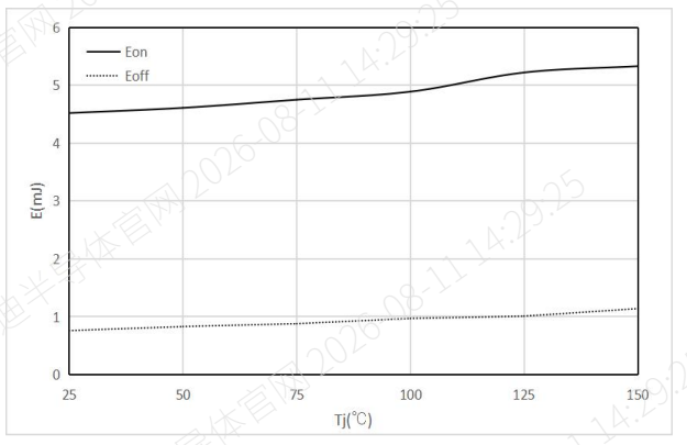
Figure 12. Typical switching energy losses as a function of junction temperature ( V_{CE}=400V , I_C=80A , V_{GE}=15V , R_G=10\Omega )
