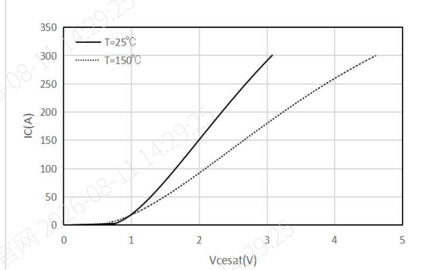
Figure 4. Typical collector current as a function of collector-emitter saturation voltage ( V_{GE}=15\text{V} )
