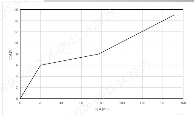
Figure 13. Typical gate charge ( V_{CE}=400V, I_C=80A )
