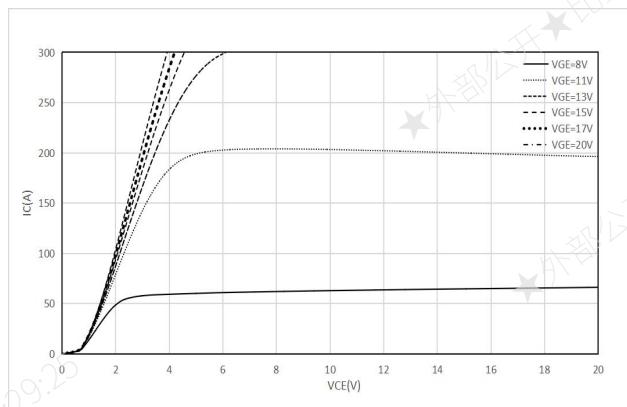
Figure 2. Typical output characteristic ( T_j=150^{\circ}\text{C} )
