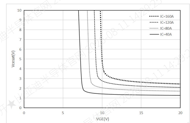
Figure 6. Typical collector-emitter saturation voltage as a function of gate-emitter voltage ( T_j=150^{\circ}\text{C} )
