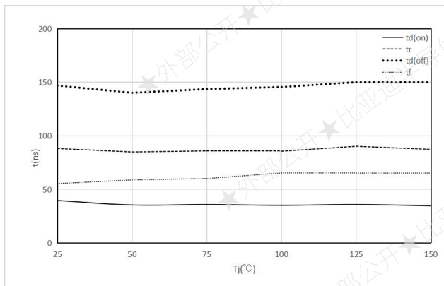
Figure 11. Typical switching time as a function of junction temperature ( V_{CE}=400V , I_C=80A , V_{GE}=15V , R_G=10\Omega )
