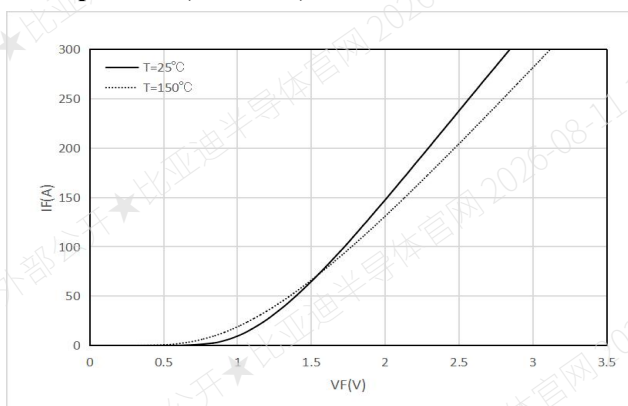
Figure 9. Typical diode forward current as a function of forward voltage
