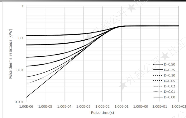
Figure 14. Transient Thermal Impedance ( D=t_p/T )
