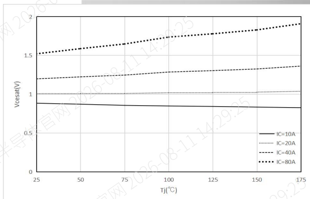
Figure 7. Typical collector-emitter saturation voltage as a function of junction temperature ( V_{GE}=15V )
