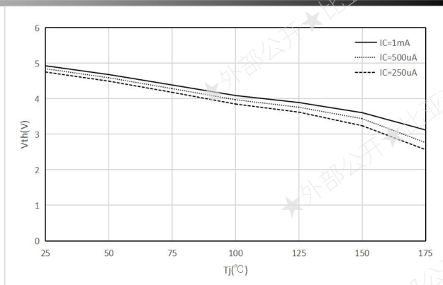
Figure 8. Gate-emitter threshold voltage as a function of junction temperature
