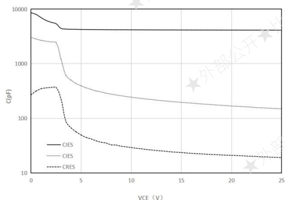
Figure 14. Typical capacitance as a function of collector-emitter voltage ( f=1MHz , V_{GE}=0V )
