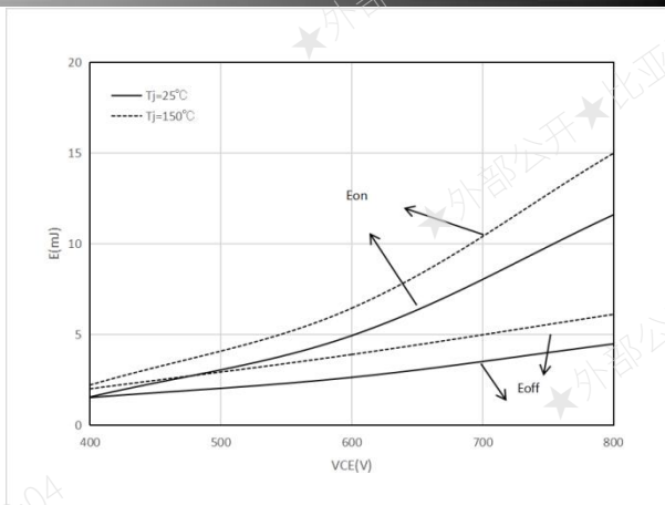
Figure 8. Typical switching energy losses as a function of collector emitter voltage ( I_C=40\text{A} , V_{GE}=15\text{V} , R_G=10\Omega )
