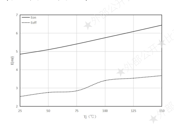
Figure 11. Typical switching energy losses as a function of junction temperature ( V_{CE}=600\text{V} , I_C=40\text{A} , V_{GE}=15\text{V} , R_G=10\Omega )
