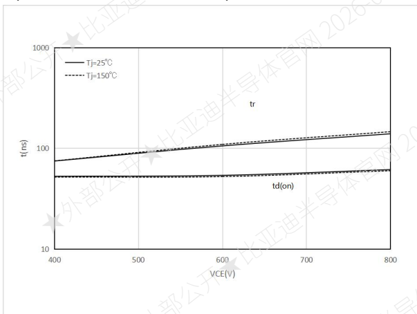
Figure 9. Typical turn-on characteristic as a function of collector emitter voltage ( I_C=40\text{A} , V_{GE}=15\text{V} , R_G=10\Omega )
