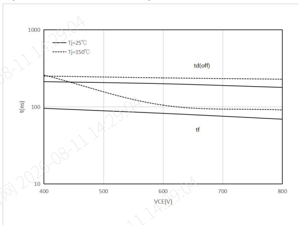
Figure 10. Typical turn-off characteristic as a function of collector emitter voltage ( I_C=40\text{A} , V_{GE}=15\text{V} , R_G=10\Omega )
