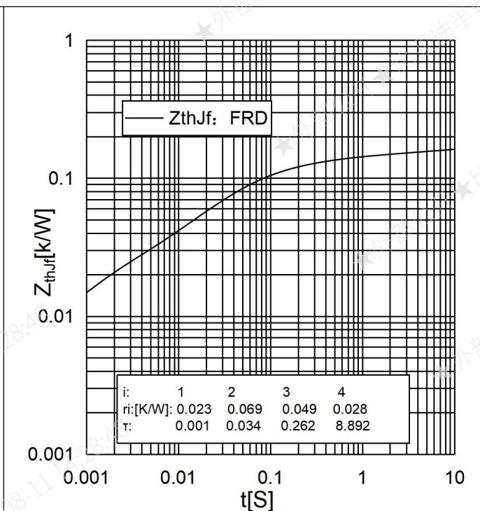
Fig.14: Typ. transient thermal impedance 图 14: 典型的瞬态热阻抗 Z_{thJf}
