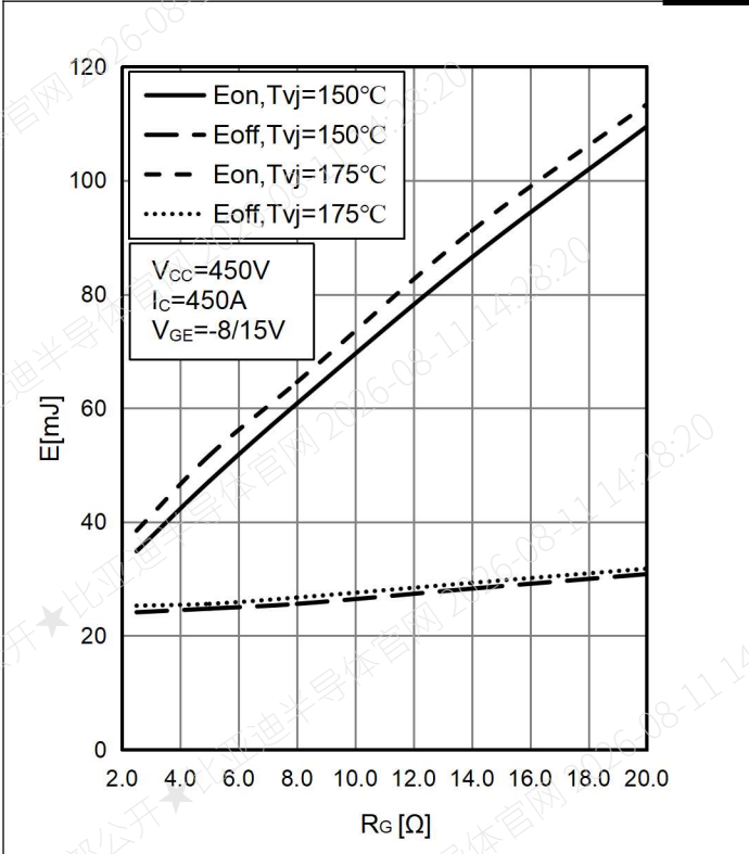
Fig.5: IGBT Switching Loss vs. R_G
