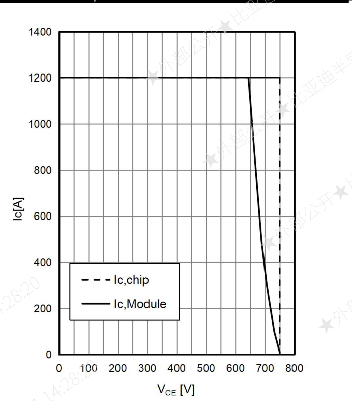
Fig.6: Reverse Bias Safe Operating Area
