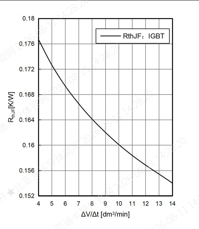
Fig.8: IGBT thermal impedance
