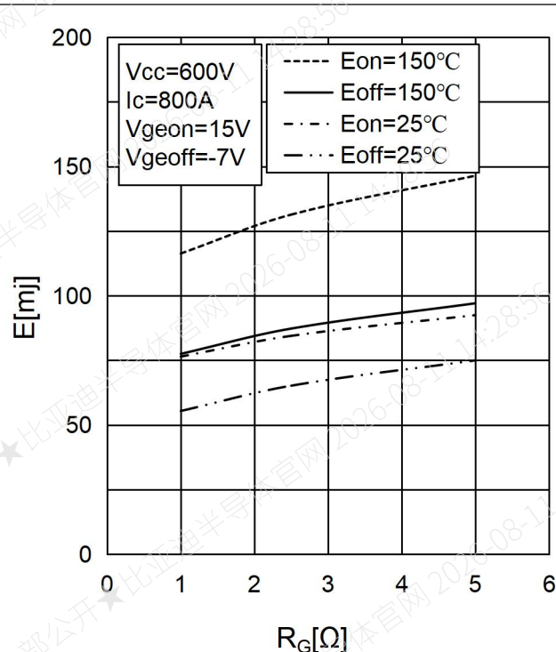
Fig.4: Switching Loss vs. Gate Resistor 图 4: 开关损耗与门极电阻关系
