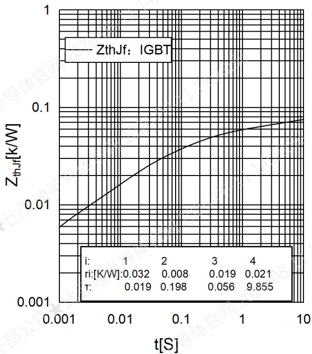
Fig.13: Typ. transient thermal impedance 图 13: 典型的瞬态热阻抗 Z_{thJf}
