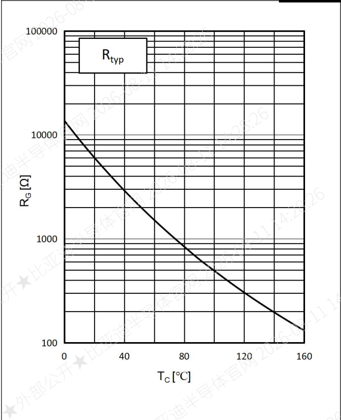
Fig.17: NTC temperature characteristic (typical)
