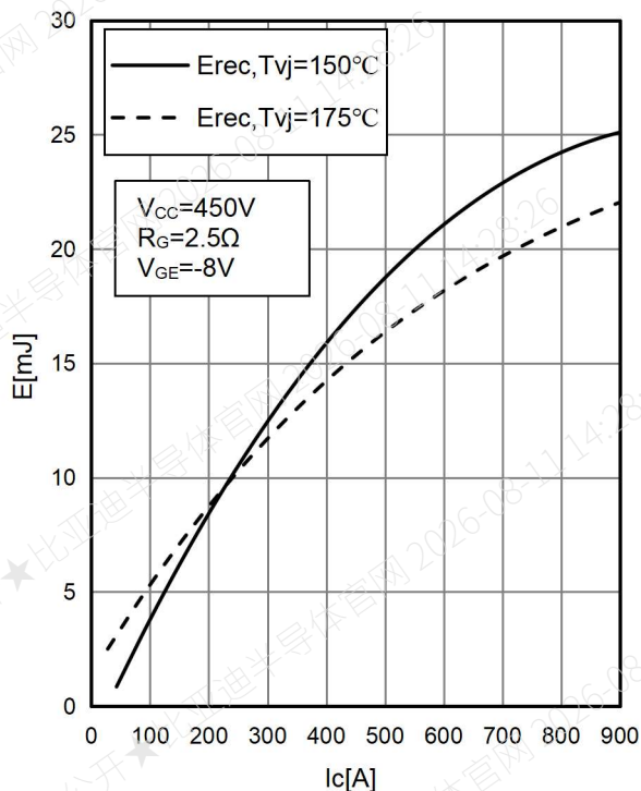
Fig.13: Diode Switching Loss vs. I_F
