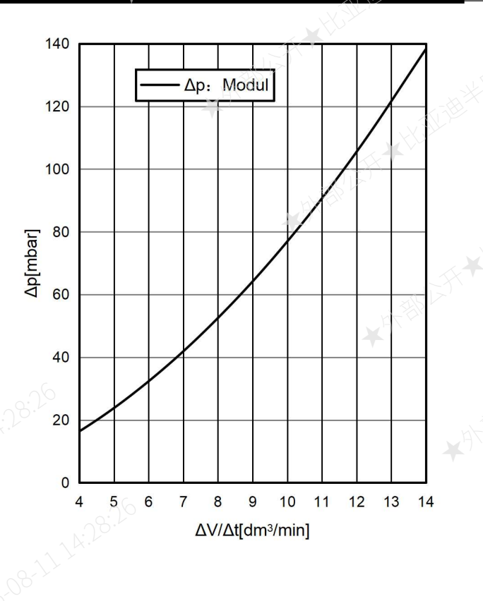
Fig.18: Pressure drop in cooling circuit
