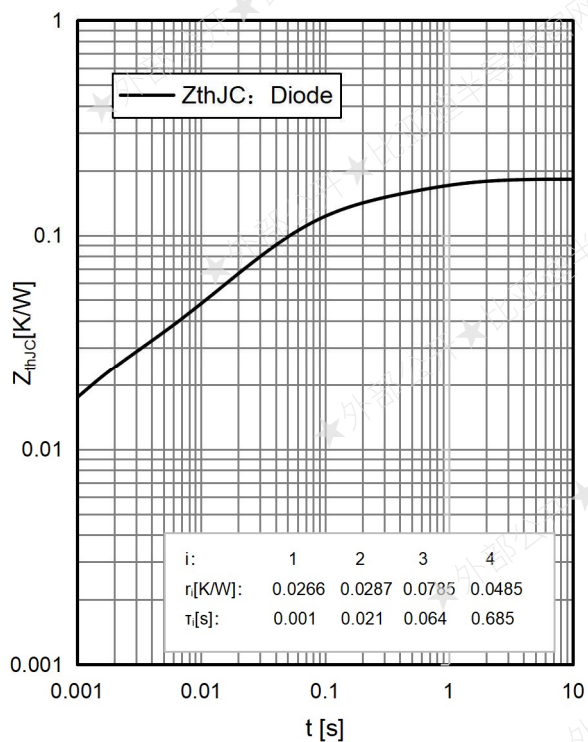
Fig.15: Diode transient thermal impedance
