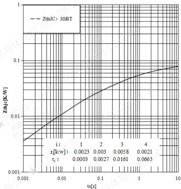
Fig.13: Typ. transient thermal impedance 图 13: 典型的瞬态热阻抗 Z_{thJC}
