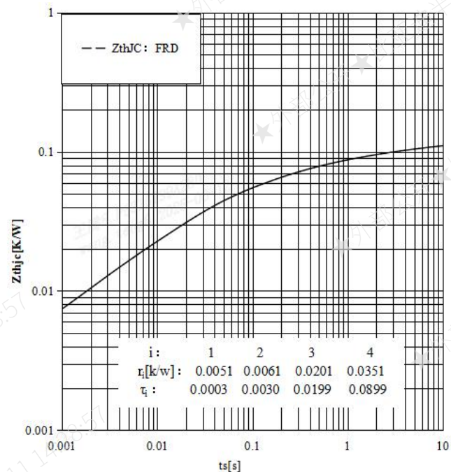
Fig.14: Typ. transient thermal impedance 图 14: 典型的瞬态热阻抗 Z_{thJC}
