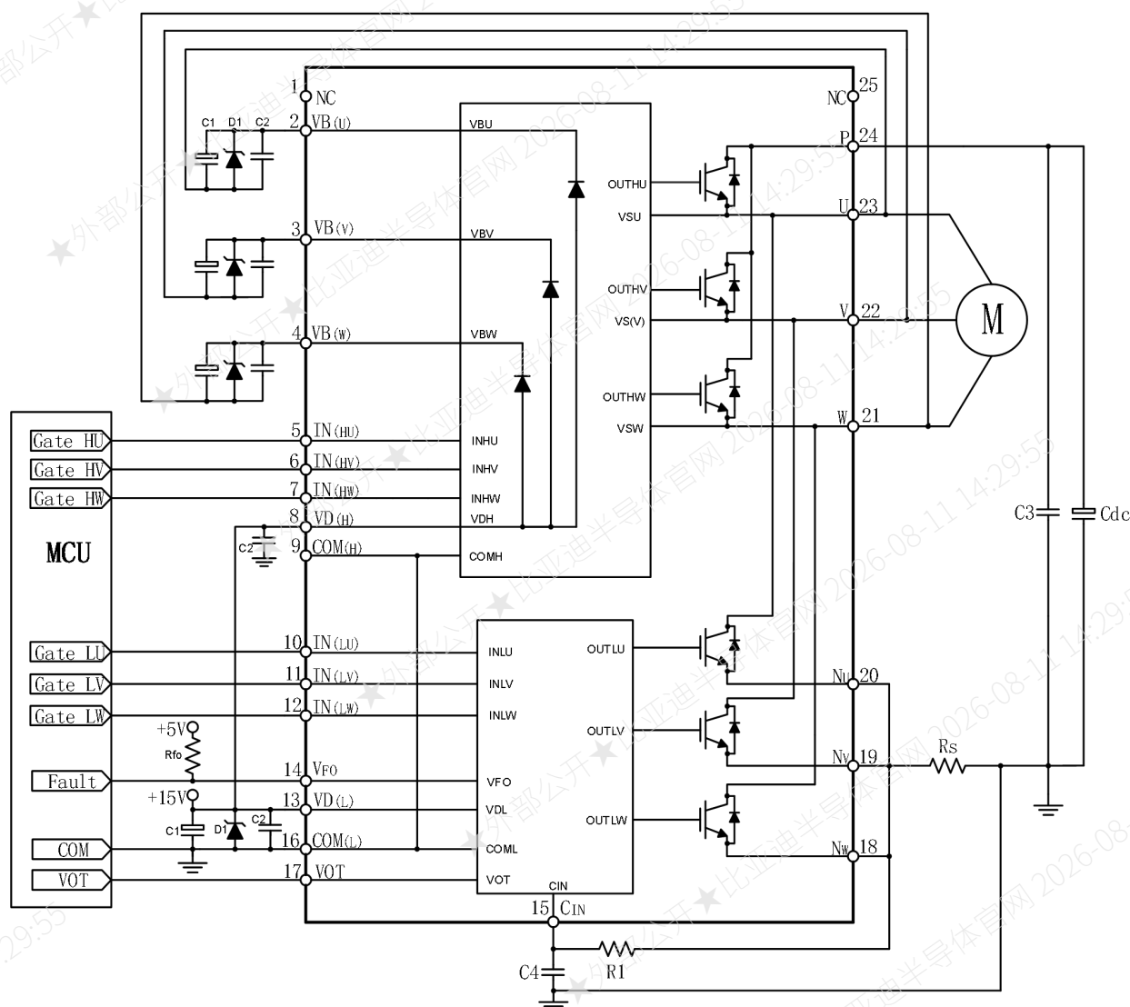
图 10.典型应用电路 Fig 10. Typical Application Circuit
